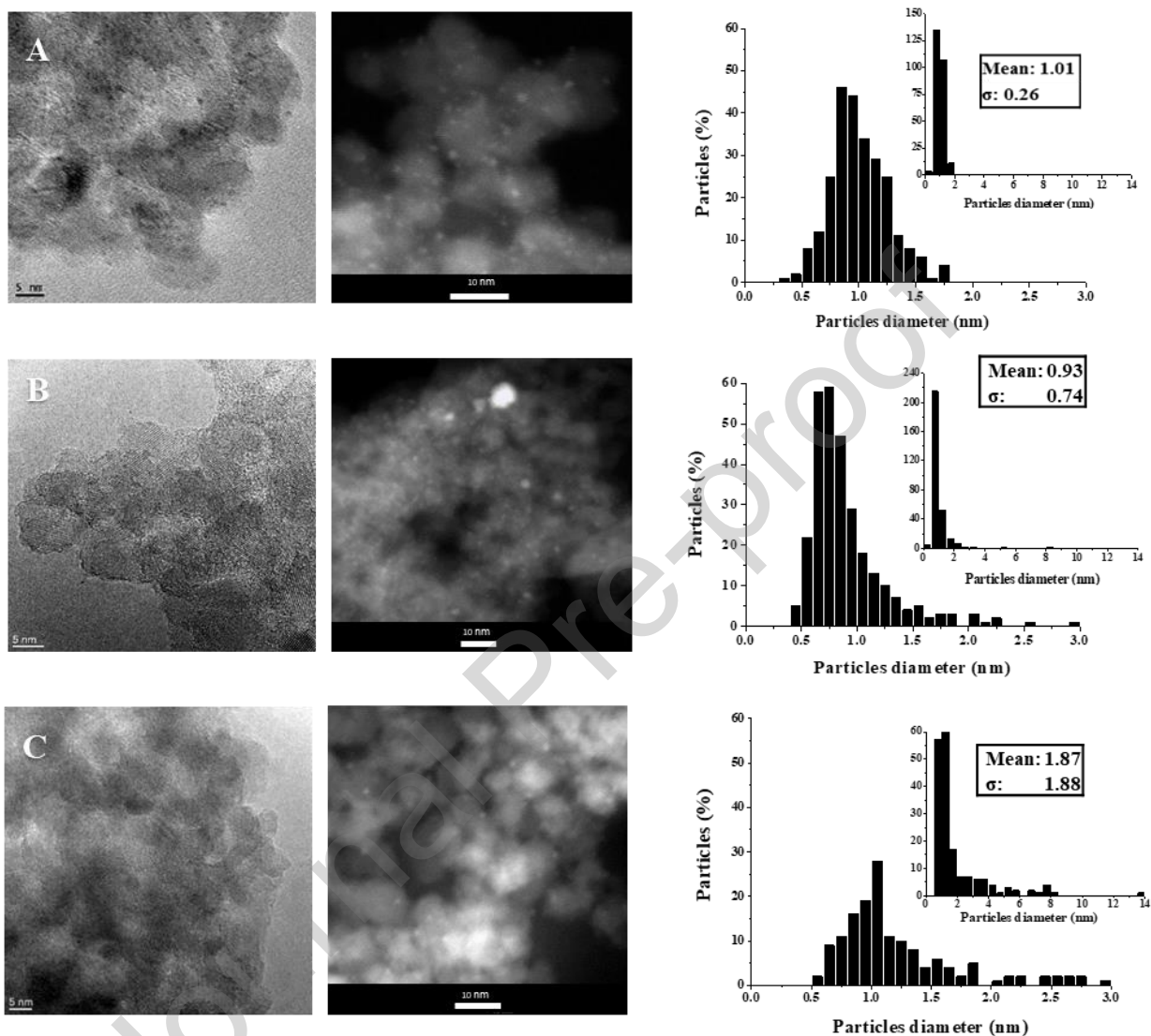
Figure 1. TEM images and particle size distribution: A) Pt/TiO 2 -m_SOMC , B) Pt/TiO 2 -m_DP , C) Pt/TiO 2 -m_IWI .
