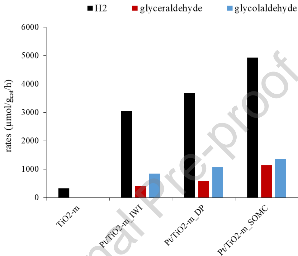
Figure 2. Rate of hydrogen production and liquid phase products for Pt NPs supported on \text{TiO}_2\text{-m} by incipient wetness impregnation (IWI), deposition-precipitation (DP) methods and Surface Organometallic Chemistry approach (SOMC). 1M aqueous solution of glycerol, 30°C; 6 h, 0.5 g/L catalyst loading.
