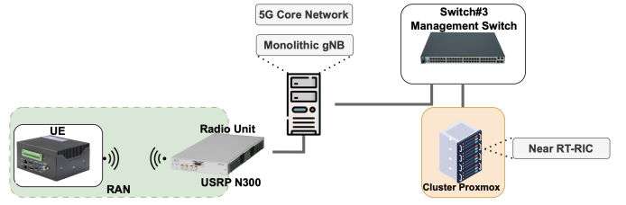
Fig. 5: Bare-Metal Deployment.
