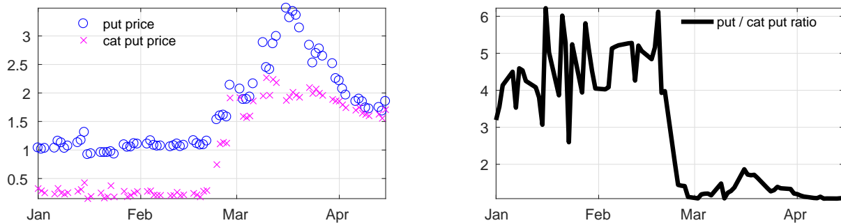
Figure 5: Monte Carlo prices of at-the-money put and cat put options with one-year maturity between January 2, 2020 to April 15, 2020.
