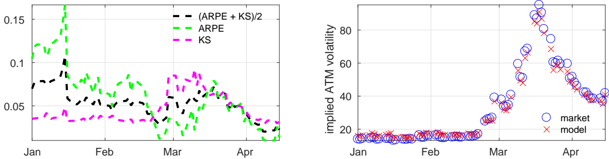
Figure 1: On the left panel, we report the implied volatility calibration error (ARPE) computed across all moneyness, the estimated KS distance and the average between the two error measures. On the right panel we report market and model at-the-money implied volatilities. The calibration was conducted for each trading day between January 2, 2020 to April 15, 2020.
