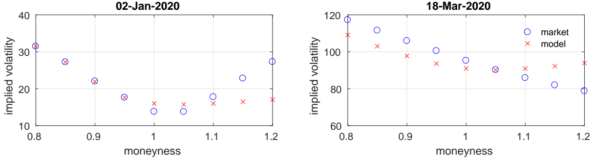
Figure 2: Calibration errors on January 2, 2020 and March 18, 2020.
