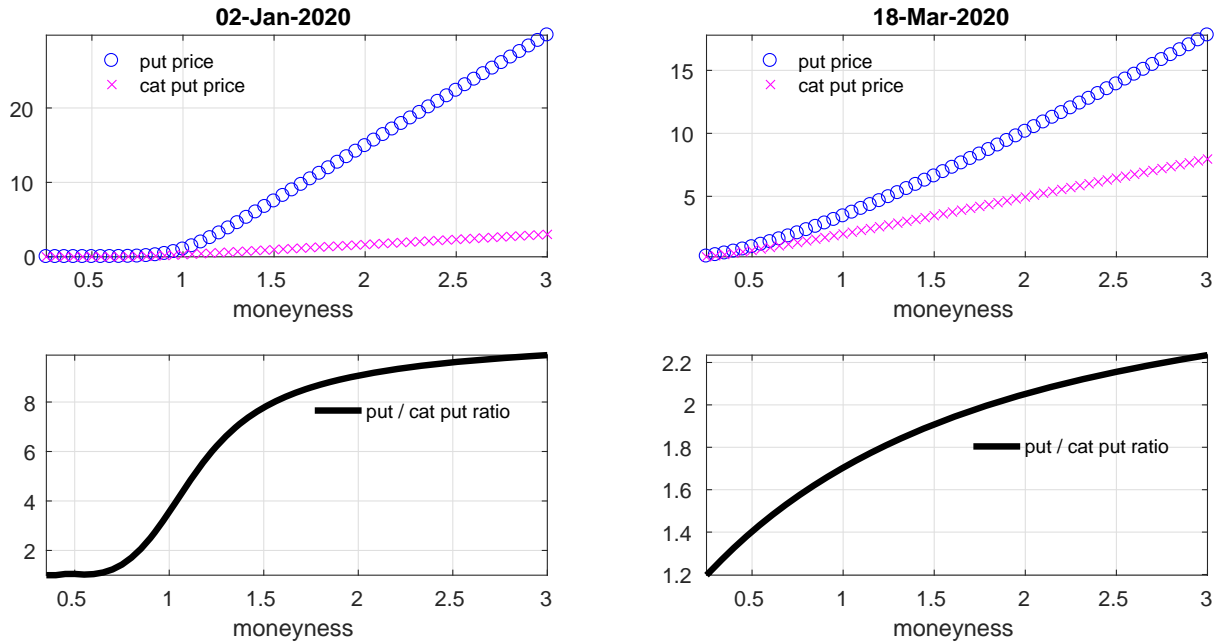
Figure 6: Monte Carlo prices of put and cat put options with one-year maturity with moneyness between 0.25 to 3 on January 2, 2020 and March 18, 2020.
