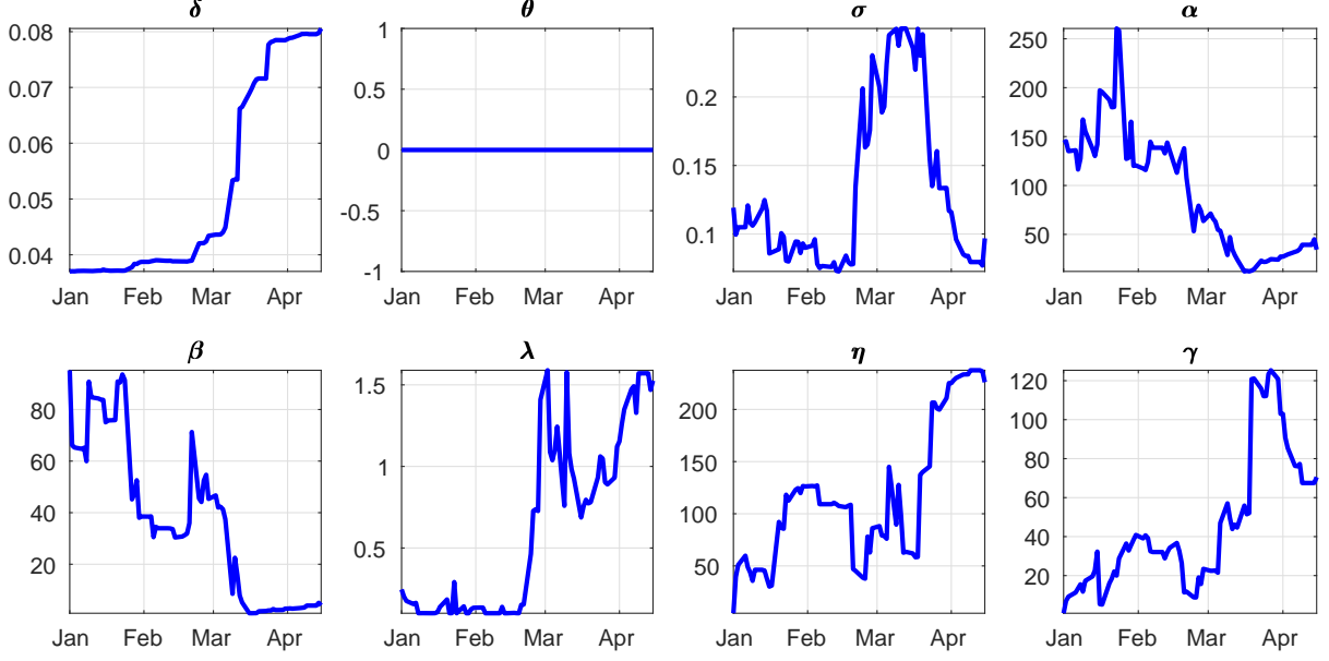
Figure 3: Risk-neutral estimated parameters. The calibration was conducted on a daily basis for each trading day between January 2, 2020 to April 15, 2020.
