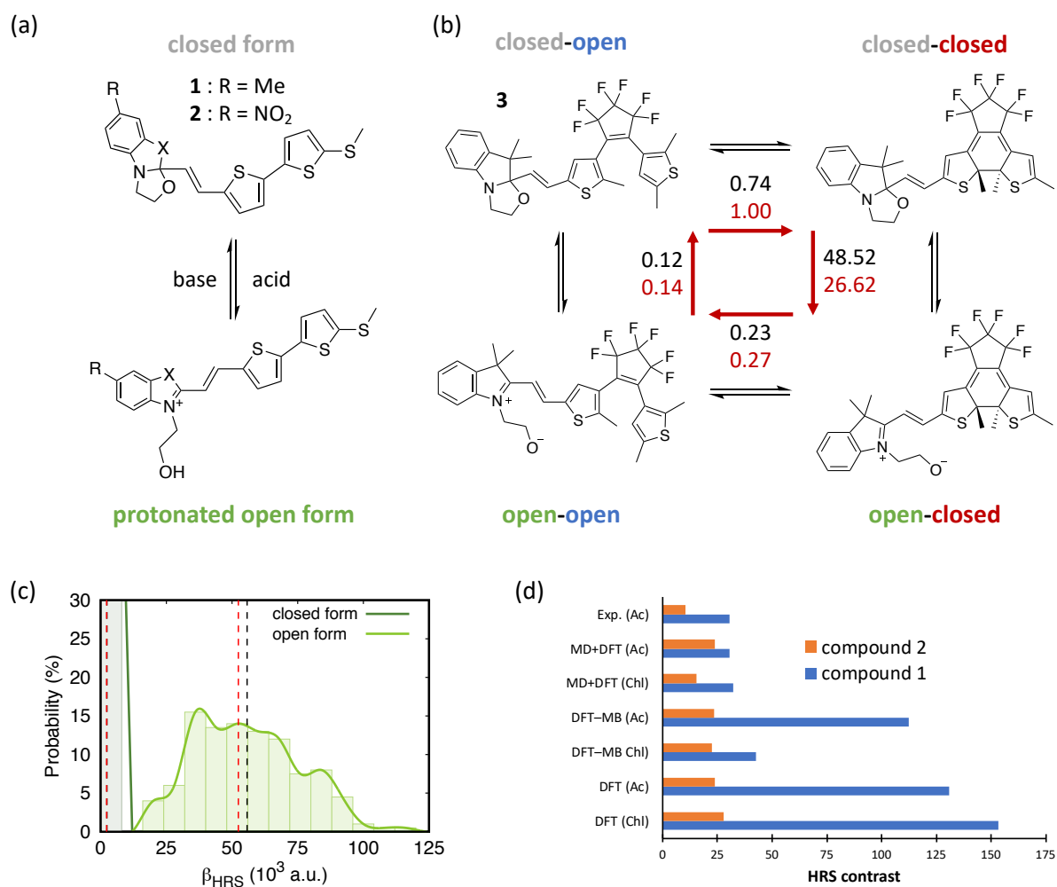
Figure 2: (a) Closed form (CF) and protonated open form (POF) of indolino-oxazolidine derivatives 1 and 2 ; (b) Interconversion scheme for biphotochromic switch 3 , with \beta_{\text{HRS}} contrasts computed using the IEF-PCM/HF (black) and MD+QM(HF) (red) levels using an incident wavelength of 1907 nm; (c) Distributions and averages of dynamic (1907 nm) \beta_{\text{HRS}} values of compound 2 computed with the MD+QM(DFT) scheme (black vertical lines) and with the DFT-MB approach (red vertical lines) in acetonitrile; (d) \beta_{\text{HRS}} contrasts upon CF \rightarrow POF switching in compounds 1 and 2 calculated in acetonitrile (Ac) and chloroform (Chl).
