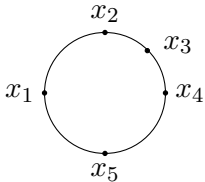
FIGURE 1. Cyclically ordered 5-tuples (x_1, \dots, x_5), (x_5, \dots, x_1)
