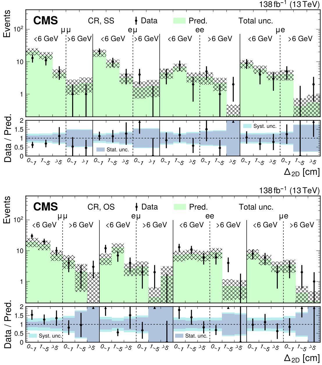
Figure 10. Predicted and observed event yields in the CR for the high-mass PFNs in the SS (upper) and OS (lower) categories, binned by flavor channel, m_{SV} (as specified below the flavor channel), and \Delta_{2D} . The hashed bands represent the total uncertainty in the background prediction. The lower panels show the data-to-prediction ratio and the background prediction uncertainty is split into statistical (“stat.”) and systematic (“syst.”) contributions.
