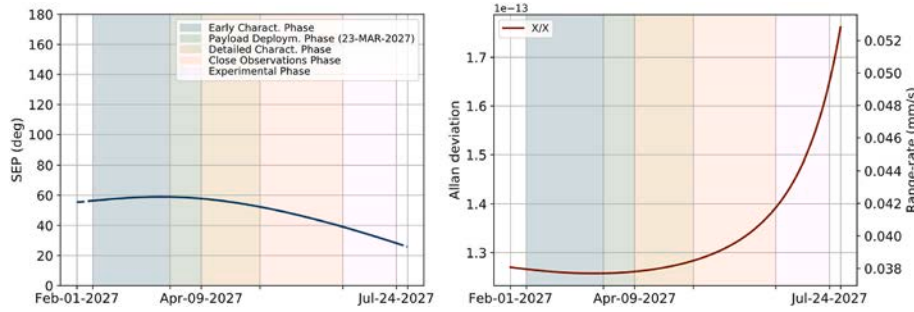
Fig. 8. Left: SEP angle during the Hera mission. Right: expected two-way Doppler noise during Hera mission at 60 s integration time. The considered noise sources are the plasma, the Earth’s atmosphere, the ground station instrumentation, and the S/C electronics. The dominant noise source is the solar plasma.
