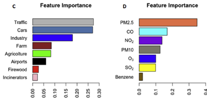
Fig. 3. Feature importance of air pollution components and its main sources for SARS-CoV-2 mortality and positivity. The feature importance produced by Random Forest model for the relation of SMR with (A) major sources, which shows that Industry, Farm and Road traffic are - respectively - the most relevant sources of air pollution connected to an increase in the mortality rates; and with (B) contaminants, which shows that PM2.5 is the most relevant component of air pollution connected to an increase in the mortality rate. The feature importance produced by Random Forest model for the relation of SPR, at the regional scale, with (C) major sources, which shows that Road traffic and Cars, Industry, and Farm are the most relevant sources of air pollution and with (D) contaminants, which shows that PM2.5, followed by CO and NO 2 are the most important components of air pollution, connected to an increase in the positivity rates.
