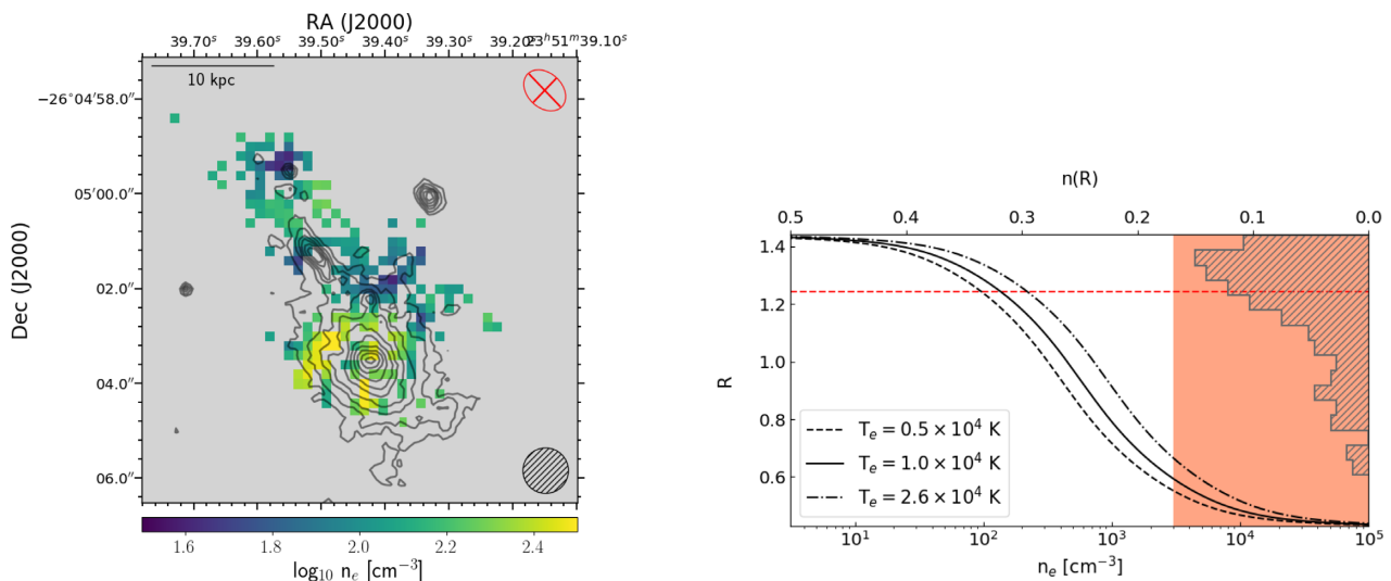
Figure 9. Left-hand panel: electron density ( n_e ) map for Abell 2667 BCG as retrieved from equation (2) for an electron temperature T_e = 1.0 \times 10^4 K, with contours and symbols as defined in Fig. 2. Right-hand panel: electron density ( n_e ) curve (Proxauf et al. 2014) as a function of the intensity ratio R = [\text{S II}] \lambda 6716/[\text{S II}] \lambda 6731 for T_e = 0.5 \times 10^4 K (black dashed line), T_e = 1.0 \times 10^4 K (black solid line), and T_e = 2.6 \times 10^4 K (black dash-dotted line). The red area of the diagram highlights the electron density values above the [S II] doublet critical density (i.e. n_e \sim 3 \times 10^3 \text{ cm}^{-3} ). We present the distribution of the retrieved R values as well as the median value of the distribution R \sim 1.21 (red dashed line).
