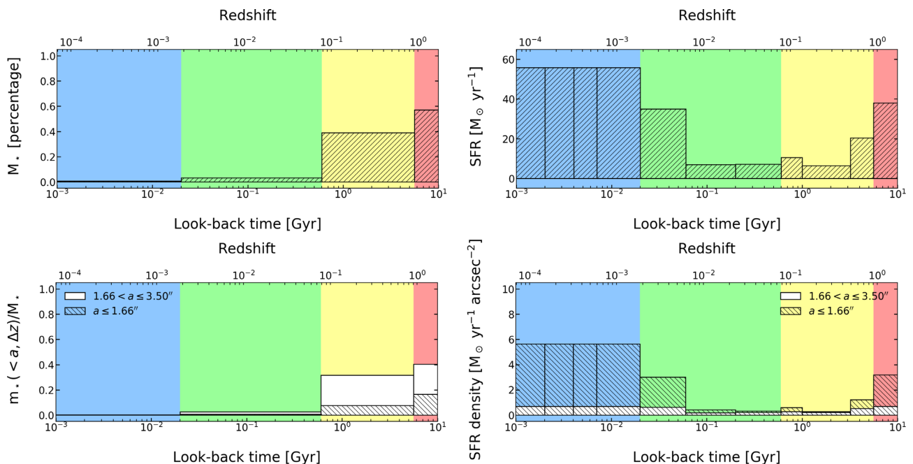
Figure 4. Top panels: SINOPSIS spatially integrated mass building ( left-hand panel ) and star formation history ( right-hand panel ) of the Abell 2667 BCG. The colour-shaded areas of the diagrams represent the four main age bins within which SINOPSIS calculates the galaxy percentage of mass built and the SFR (see Fig. 3). In the right-hand panel, the histogram show the SFH computed in the highest temporal resolution mode (11 SSP age intervals). Both the percentage of mass built and the SFR of each time-bin have been obtained integrating all the maps’ values within an elliptical region centred at the galaxy coordinates, with axis ratio b/a = 0.76 , position angle PA = 48.89^\circ (for the parameters see Section 3.1), and semimajor axis a = 3.5 arcsec. Bottom panels: percentage of stellar mass built ( left-hand panel ) and SFR density ( right-hand panel ) at different epochs for the nuclear ( hatched histogram ) and external regions ( white histogram ) of the BCG. For the nuclear region we have integrated SINOPSIS spatially resolved values within an elliptical aperture centred at the galaxy coordinates, with b/a and PA as before but a = 1.66 arcsec. For the outskirts, we have resorted to an elliptical annulus with central coordinates, b/a and PA as before, but with 1.66 \text{ arcsec} < a \leq 3.55 \text{ arcsec} . The two different areas are marked with the two white ellipses in the top left-hand panel of Fig. 3.
