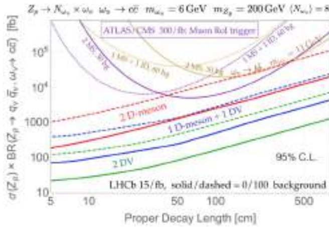
Figure 54. Projected bounds from various proposed searches for confining hidden valley models exploiting c\bar{c} decays of hidden valley mesons \omega_V (taken from [383]). The sensitivities with various signatures at LHCb are shown: two displaced vertices (green), one reconstructed D meson and one DV (blue) and two reconstructed D mesons (red). Searches for this same particular model at ATLAS/CMS are shown not to be competitive (more details can be found in [383]).
