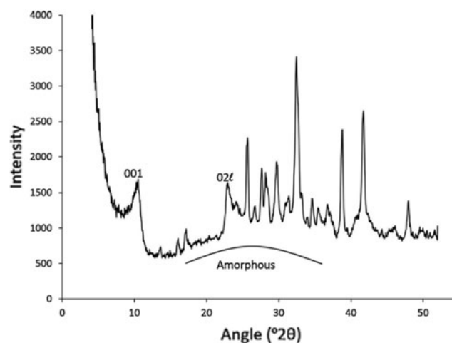
FIG. 10. A CheMin X-Ray diffraction pattern of the Marimba sample from the Murray formation, Gale Crater. The broad increase in the baseline between 18 and 35° 2θ is attributed to the presence of X-ray amorphous phases. 001 and 02l refer to diffraction peaks attributed to clay minerals. Figure adapted from Rampe et al. (2020).
