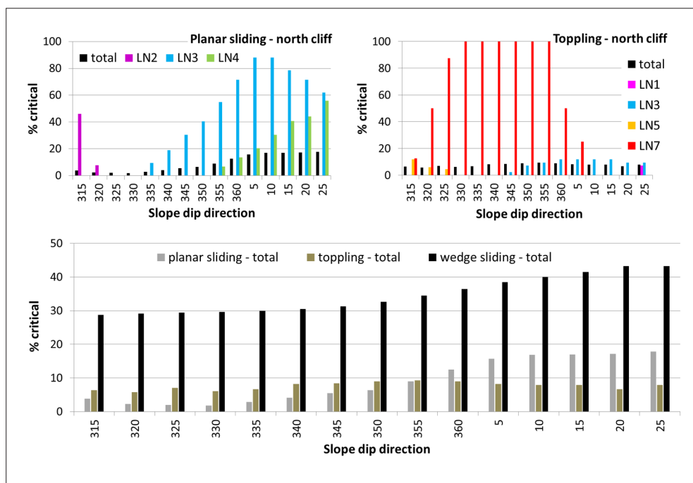
Figure 11 - Representation of the percentage of discontinuity poles included in the critical area for different slope dip directions (slope dip was fixed to 90°). The percentage was calculated separately for each joint set (number of critical joint in set N/total number of joint in set N) and considering the amount of all the mapped discontinuities (total).
