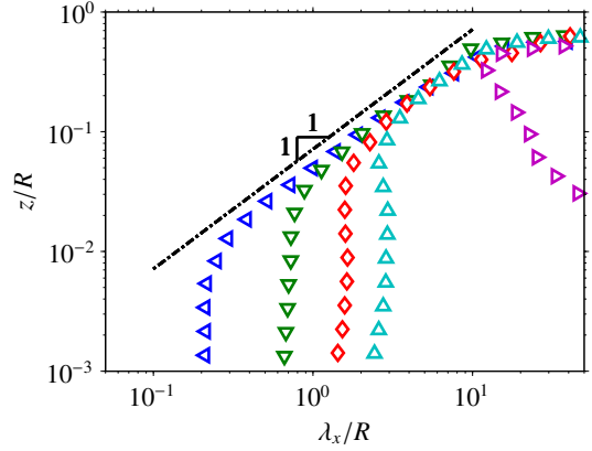
Figure 13: \gamma_L^2 = 0.1 contours between u and u_\tau signals at Re_\tau \approx 40\,000 as function of \Delta s ; \Delta s/R \approx 0 ( \triangleleft ), 0.02 ( \nabla ), 0.03 ( \diamond ), 0.06 ( \triangle ) and 0.13 ( \triangleright ).
