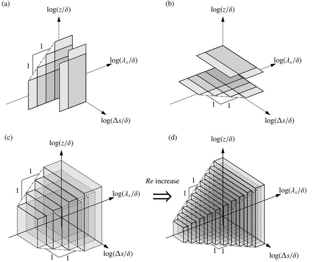
Figure 15: A model for \gamma_L^2 following the attached eddy hypothesis. (a-c) Correspond to the case with four hierarchy levels, with (a) and (b) showing \gamma_L^2 at a constant \Delta s and z , while (c) illustrates the iso-contours of \gamma_L^2 as functions of \lambda_x , \Delta s and z . Meanwhile, (d) shows the iso-contours for the case with ten hierarchy levels, which corresponds to a higher Re scenario.
