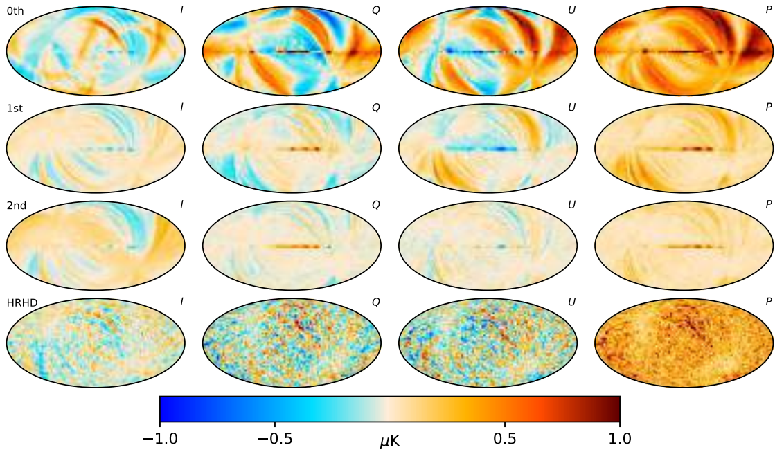
Fig. F.1. Simulated full-mission maps of HFI ADCNL at 143 GHz. Top row : full, unmitigated effect. Second row : residuals after fitting and correcting ADCNL using the linear gain model (first-order correction), as was done in PR3. Third row : residual after fitting for gain and distortion terms, as is done in NPIPE. The NPIPE transfer function (Sect. 4.3) applies to both the full and ADCNL-free simulations. Fourth and last row : half-ring, half-difference map from the same simulation to compare the magnitude of the effect to instrumental noise. All maps were smoothed with a 3^\circ Gaussian beam. The residual power spectra are shown in Fig. F.2.
