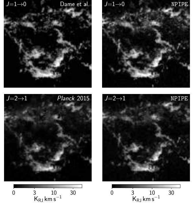
Fig. 64. 30° × 30° expansion of various CO emission line maps. All maps are smoothed to 14' FWHM and are centred on the Orion region, with Galactic coordinates ( l, b ) = (210°, −9°).
