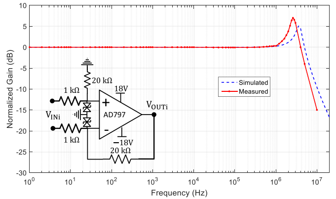
Fig. 5. Simulated (dashed blue line) and measured (continuous red line) small-signal gain (normalized) of a 20\times voltage amplifiers. The -3\text{-dB} bandwidth is about 6 MHz and the in-band ripple is lower than 0.03 dB up to 1 MHz.
