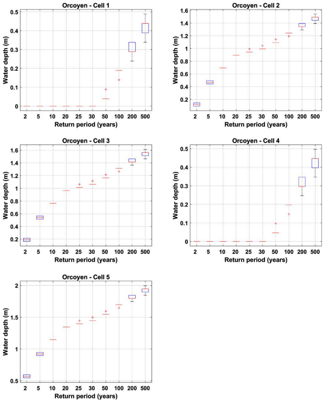
Fig. 17. Uncertainty in T-year water depths obtained by using the stochastic methodology. Red lines represent the median. Blue boxes represent 25th and 75th percentiles. Red crosses represent outliers.
