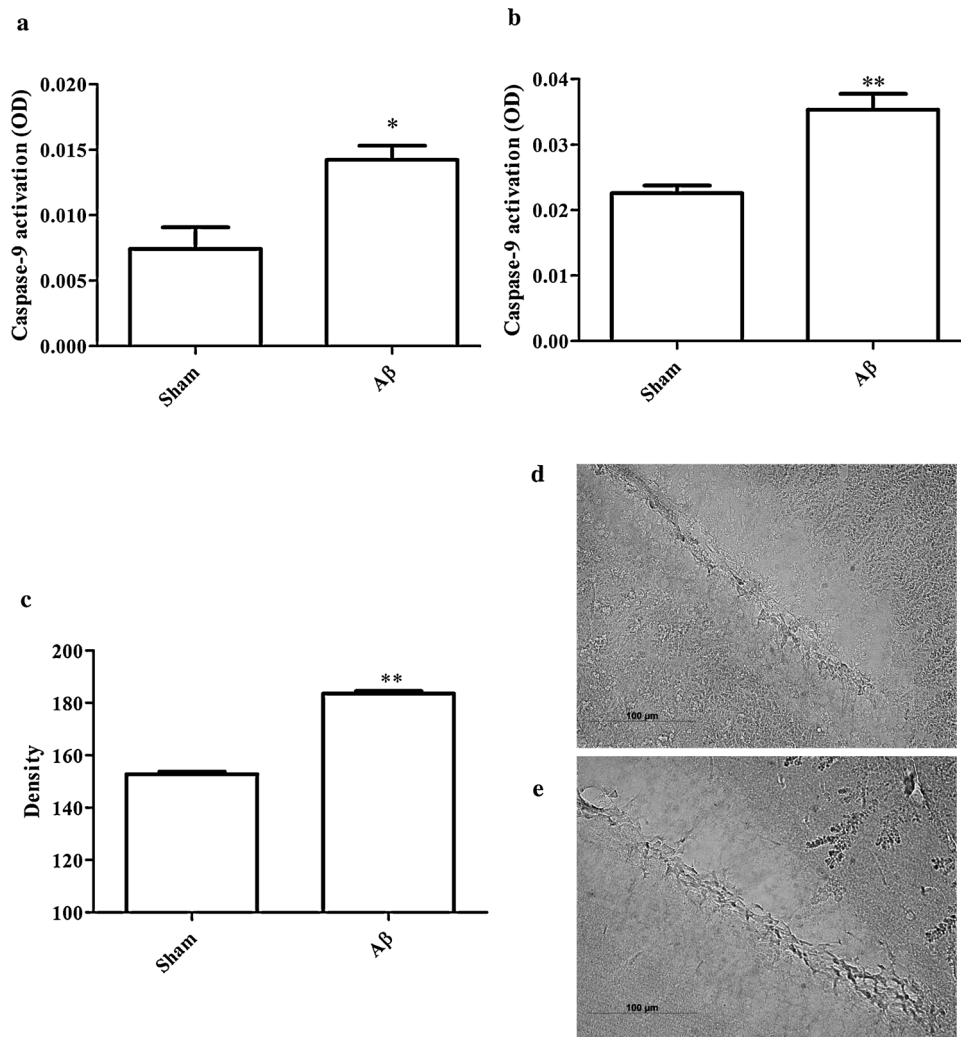
Fig. 4. Effects of A\beta_{1-42}O injection on caspase-9 activation. Caspase-9 activity was determined using specific chromogenic substrate in the hippocampus (a) and cerebral cortex (b). Values are expressed as mean \pm SEM ( n = 10 ) of optical density (OD) of each experimental group (a: * p < 0.05 vs sham group; b: ** p < 0.01 vs sham group; t -test). Caspase-9 immunoreactivity was performed in hippocampal sections. Quantitative analysis of caspase-9 immunostaining (c). Representative photomicrographs of immunostaining for cleaved caspase-9 in brain coronal sections containing hippocampal structure of sham (d) and A\beta (e) mice. Scale bar 100 \mu m . Values are expressed as mean \pm SEM ( n = 10 ) of the density of each experimental group (c: ** p < 0.01 vs sham group; t -test).
