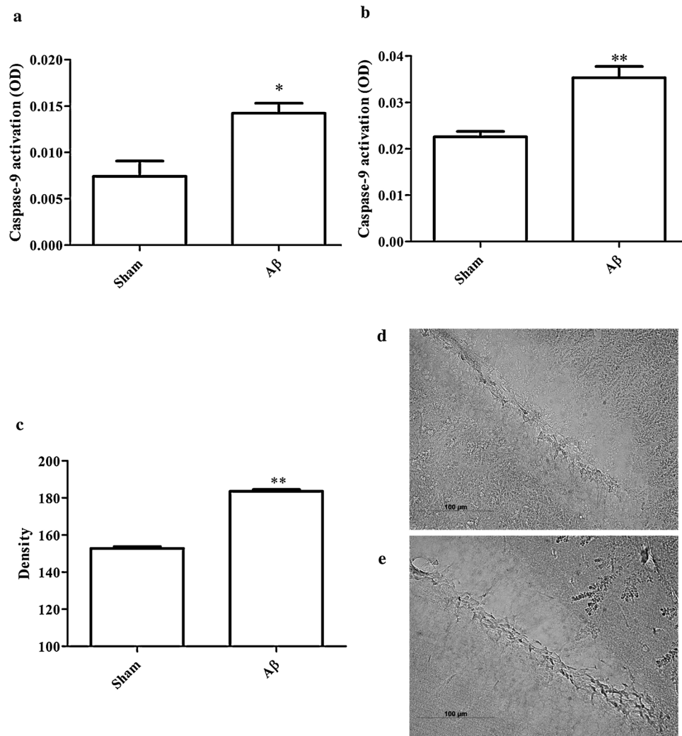
Fig. 4. Effects of Ab 1-42 O injection on caspase-9 activation. Caspase-9 activity was determined using specific chromogenic substrate in the hippocampus (a) and cerebral cortex (b). Values are expressed as mean \pm SEM ( n = 10 ) of optical density (OD) of each experimental group (a: * p < 0.05 vs sham group; b: ** p < 0.01 vs sham group; t -test). Caspase-9 immunoreactivity was performed in hippocampal sections. Quantitative analysis of caspase-9 immunostaining (c). Representative photomicrographs of immunostaining for cleaved caspase-9 in brain coronal sections containing hippocampal structure of sham (d) and Ab \beta (e) mice. Scale bar 100 \mu m. Values are expressed as mean \pm SEM ( n = 10 ) of the density of each experimental group (c: ** p < 0.01 vs sham group; t -test).
