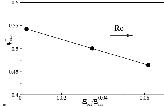
FIGURE 6. Behavior of the near-wall peak of the single point spatial flux, \psi_{max}^+ , equation (2.1), as a function of the ratio \Xi_{out}/\Xi_{inn} for increasing Reynolds number.
