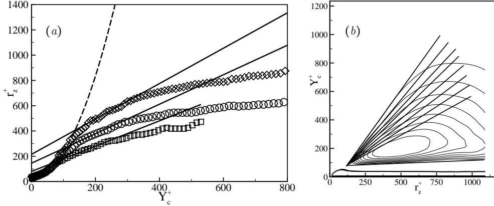
FIGURE 5. (a) Spanwise scale of maximum scale-energy source, (\ell_z^{\max})^+ , as a function of the wall distance. Diamonds denote the Re_\tau = 1500 case, circles the Re_\tau = 1000 case and squares the Re_\tau = 550 case. The dashed line denotes the quadratic increase near the wall, (\ell_z^{\max})^+ = 35 + 0.02Y_c^{+2} while the solid lines the linear increase in the overlap layer, (\ell_z^{\max})/h = 0.14 + (Y_c/h) , (\ell_z^{\max})/h = 0.14 + 1.16(Y_c/h) and (\ell_z^{\max})/h = 0.14 + 1.4(Y_c/h) , expressed in viscous units, i.e. (\ell_z^{\max})^+ = 80 + Y_c^+ , (\ell_z^{\max})^+ = 145 + 1.16Y_c^+ and (\ell_z^{\max})^+ = 215 + 1.4Y_c^+ . (b) Energy source -\xi^+ isolines in the r_x = 0 plane for the Re_\tau = 1500 case. The straight lines are r_z^+ = \gamma(\xi_0^+)(Y_c^+ - \tilde{Y}_c^+) + \tilde{r}_z^+ where \xi_0^+ defines the iso-level of \xi , \gamma(\xi_0^+) \in [0.04, 1.4] , \tilde{r}_z^+ = 120 and \tilde{Y}_c^+ = 80 .
