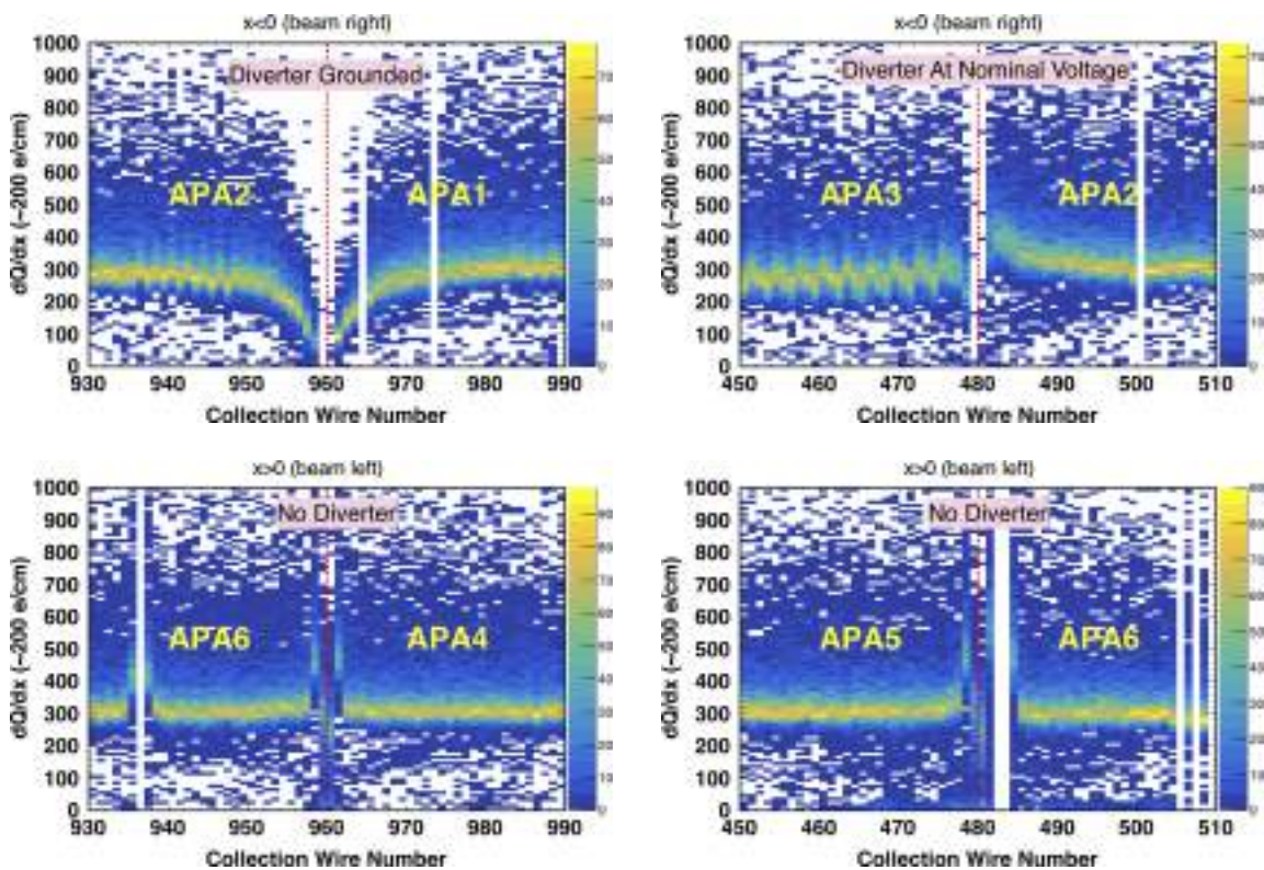
Figure 2.24. The dQ/dx distributions as a function of the collection wire number zoomed in near the gaps, using cosmic ray muons in ProtoDUNE-SP run 5924. The electron diverters are only instrumented for the gaps at the beam right side ( x < 0 ). The electron diverter between APA 2 and APA 3 was running at the nominal voltage while the electron diverter between APA1 and APA 2 was turned off.
