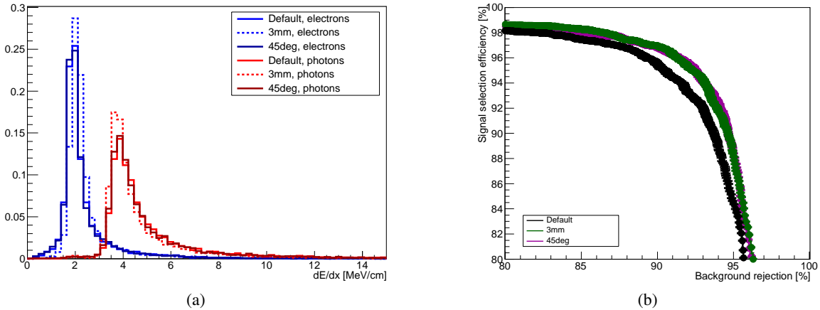
Figure 2.5. Summary of electron-photon separation performance studies from the DUNE FD task force. (a) e-\gamma separation by dE/dx for the nominal wire spacing and angle ( 4.7\text{ mm}/37.5^\circ ) compared to 3\text{ mm} spacing or 45^\circ induction wire angles. (b) Electron signal selection efficiency versus photon (background) rejection for the different detector configurations. The 3\text{ mm} wire pitch and 45^\circ wire angle have similar effects, so the 45^\circ curve is partly obscured by the 3\text{ mm} curve.
