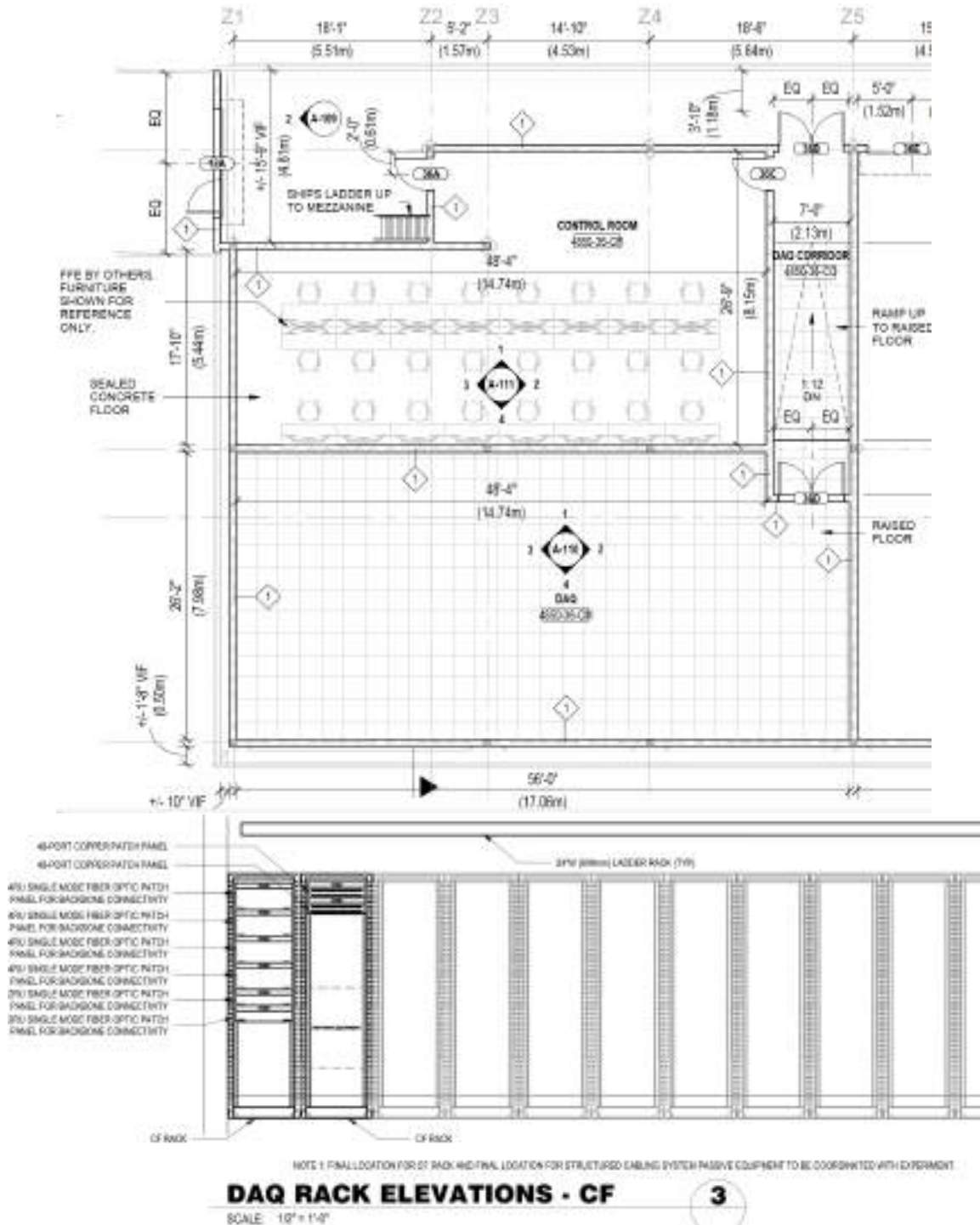
Figure 9.23. Top: the overall layout of the DUNE spaces in the CUC. A110 is the DUNE data room, which houses the underground computing, and A111 is a general-purpose work area (not a control room, as labeled) that we call the experimental work area. Bottom: the first row of ten racks in the data room is shown. The first two represent the CF interface racks. The images were taken from the ARUP 90% design drawings U1-FD-A-108 and U1-FD-T-701 [157].
