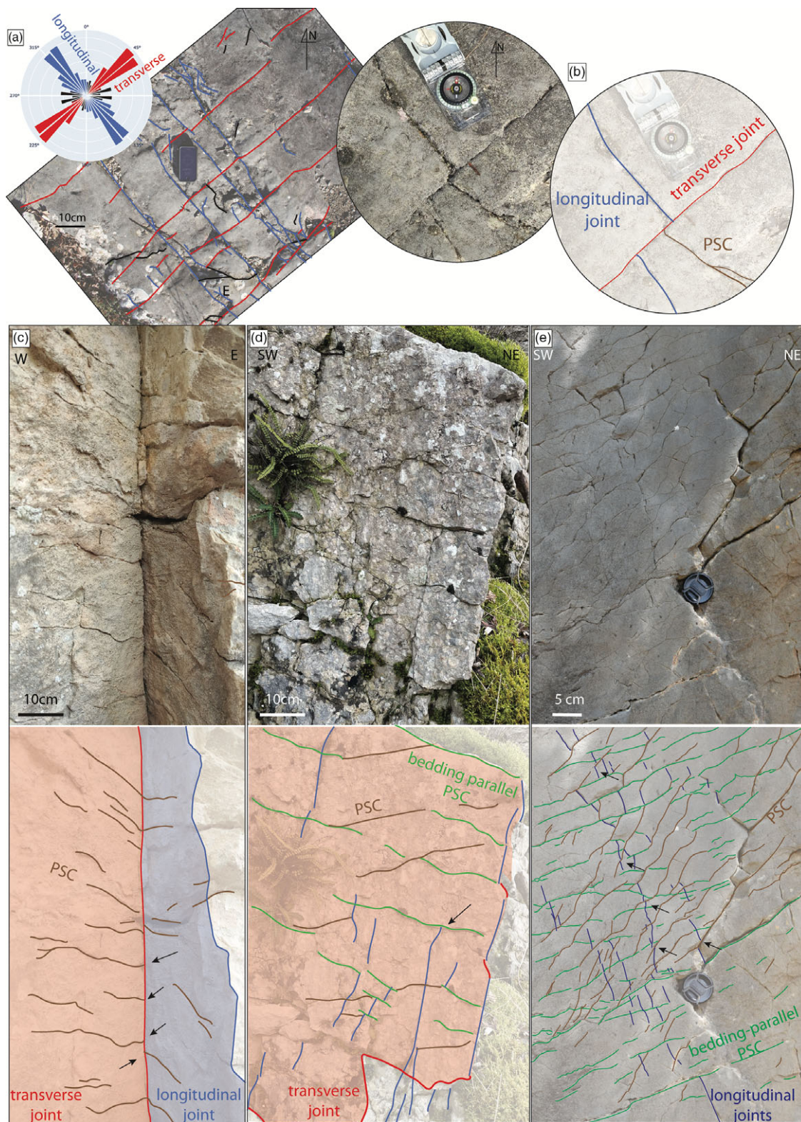
Fig. 6. (Colour online) Cross-cutting relationships. (a) Scan area and related rosettiagram showing mutual cross-cutting relationships between two joint sets. (b) The trace of a pressure-solution cleavage abuts on a joint. (c) Pressure-solution cleavages oriented oblique to bedding both cross and abut on (see black arrow) a joint. (d) Joints abut on bedding-parallel pressure-solution cleavages (black arrow). (e) A longitudinal joint is deformed by pervasive pressure-solution cleavage. Black arrows indicate portions of the outcrops where the joint is dislocated by pressure-solution cleavage.
