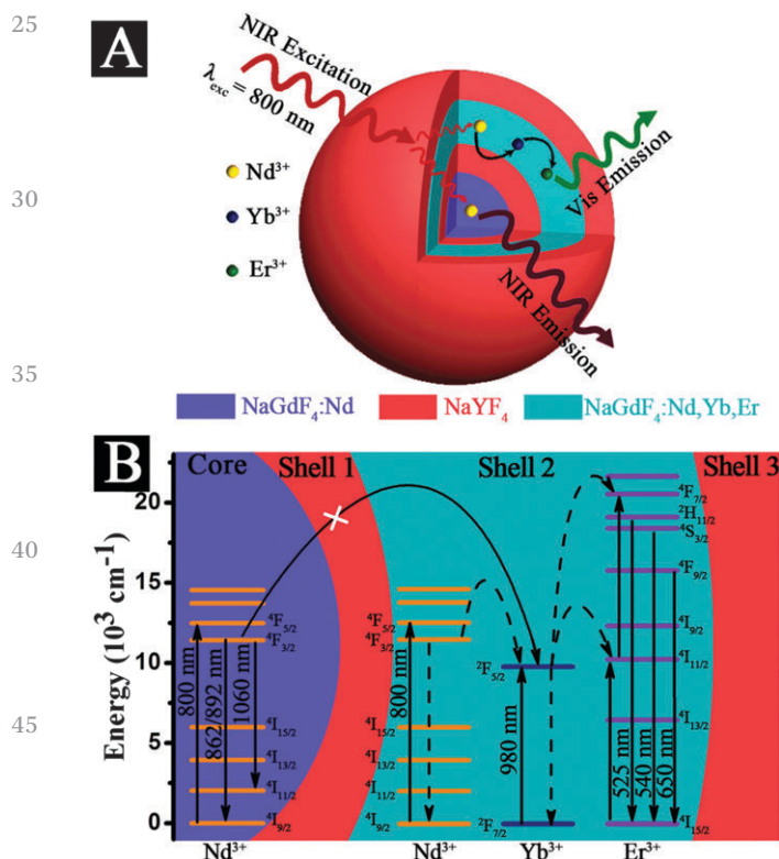
Fig. 14 (A) General strategy to achieve the UC and DS dual-mode luminescence with multi-layer C/S1/S2/S3 β-NaGdF 4 :Nd/NaYF 4 /NaGdF 4 :Nd,Yb,Er/NaYF 4 NPs. (B) Proposed energy transfer mechanisms in the multi-layer core-shell NPs. Adapted from ref. 109 Copyright 2013 Macmillan Publishers Limited.
