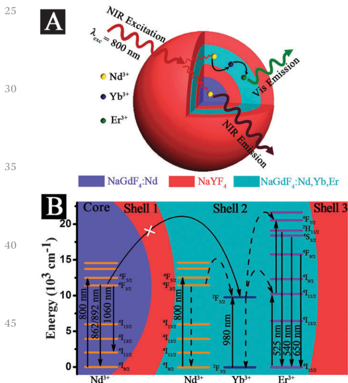
Fig. 14 (A) General strategy to achieve the UC and DS dual-mode luminescence with multi-layer C/S1/S2/S3 \beta -NGdF 4 :Nd/NaYF 4 /NaGdF 4 :Nd,Yb,Er/NaYF 4 NPs. (B) Proposed energy transfer mechanisms in the multi-layer core-shell NPs. Adapted from ref. 109 Copyright 2013 Macmillan Publishers Limited.
