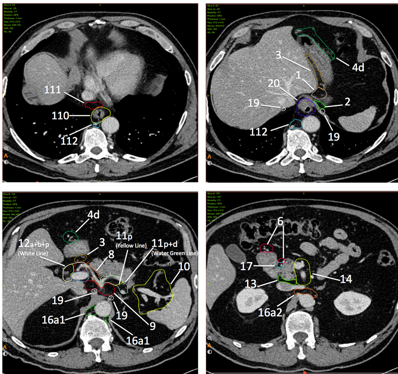
Fig. 1. Example of atlas of LN's delineation validated by the WG.
