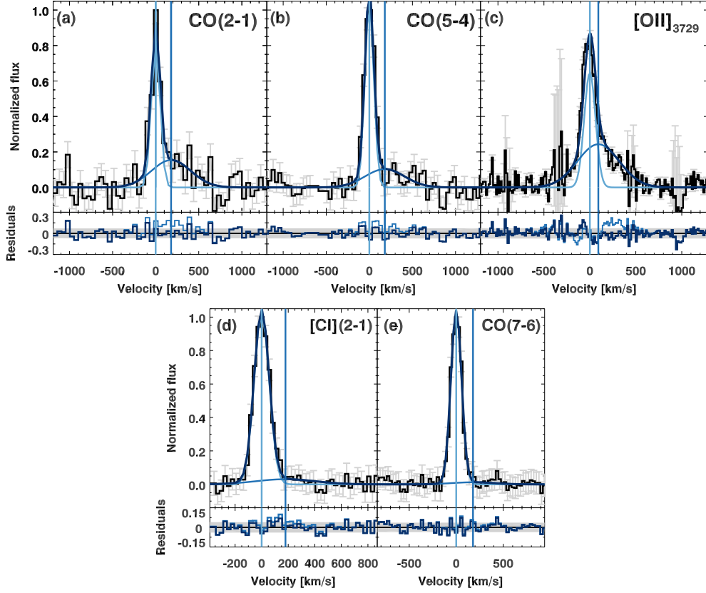
Figure 1: Multi-wavelength spectra of ID2299. Panel a-e: CO(2-1), CO(5-4), [OII] 3729 , [CI](2-1) and CO(7-6) spectrum of the source. To aid the visual comparison with the CO/[CI] spectra, in panel c the \lambda_{\text{rest}} = 3726 Å narrow+broad Gaussian model has been subtracted from the observed spectrum and only the \lambda_{\text{rest}} = 3729 Å narrow+broad complex of the [OII] 3726,3729 doublet is shown. The spectra are continuum-subtracted and are centred to the systemic velocity of the galaxy. The spectra are also normalized to the peak of the narrow emission. In all top panels the black curve and the light grey errorbars represent the observed flux and 1\sigma uncertainty, respectively. Here, light blue lines show the Gaussian fits to the narrow and broad component. The darkest blue curve represents the total fit. Solid vertical lines mark the centroids positions. Below each spectrum, light and dark blue curves show relative residuals from a single and a two Gaussian fit, respectively. Here, light gray horizontal areas highlight the RMS level of the single Gaussian fit residuals.
