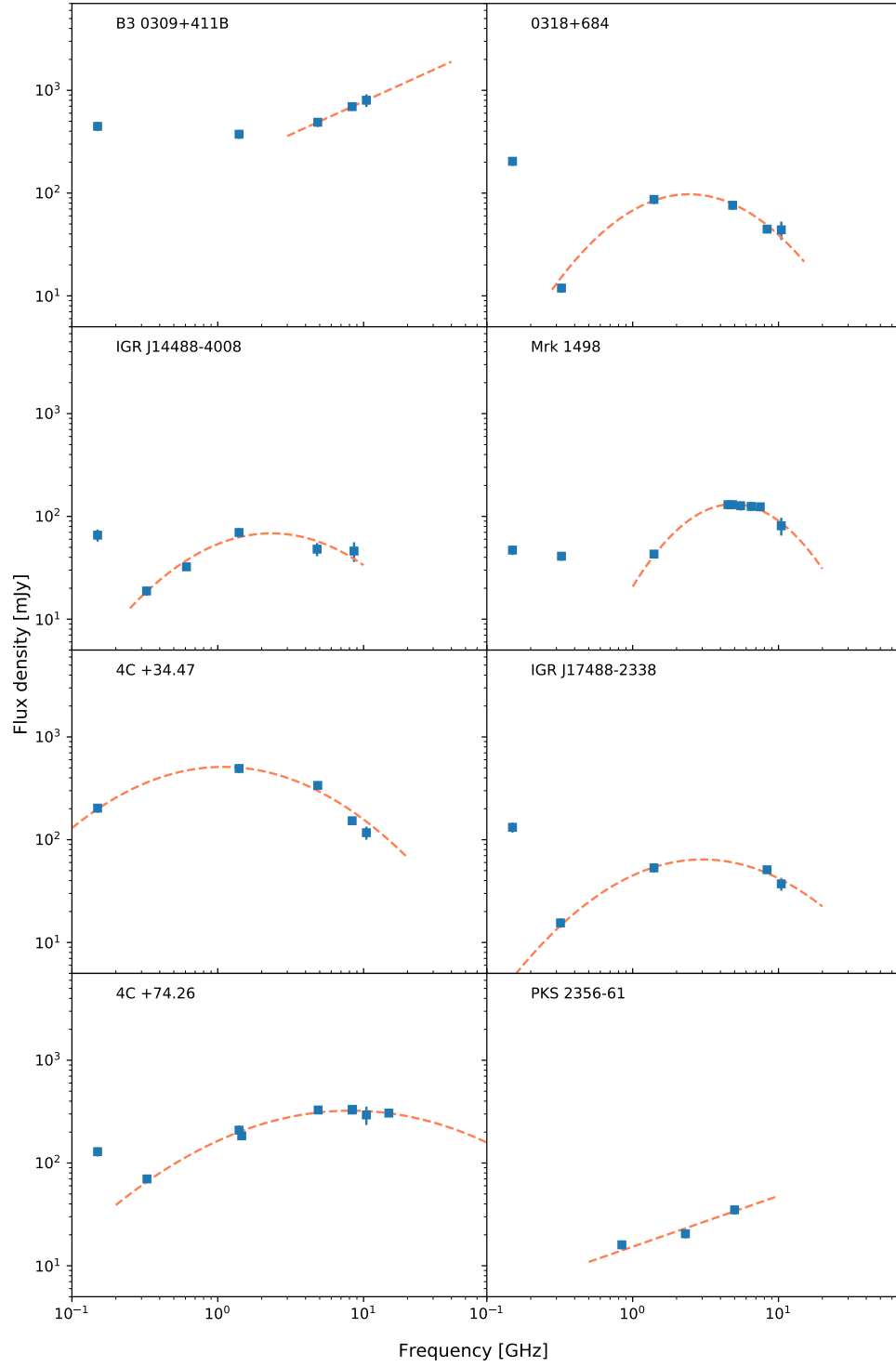
Figure 1. GPS radio cores spectra. Errors in logarithmic scale are smaller than symbol size for most of measurements. The point at 250 GHz for 4C +74.26 is out of scale.
