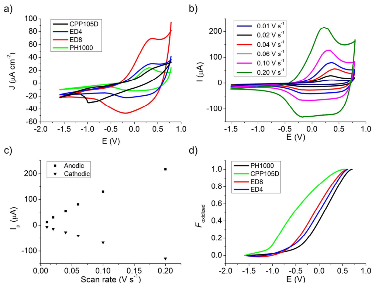
Figure 1. a) CVs recorded for different PEDOT:PSS substrates (scan rate 20 \text{ mV s}^{-1} ). b) Cyclic voltammograms of PH1000 taken at different scan rates. c) Peak current vs. scan rate. d) Fraction of oxidized PEDOT:PSS ( F_{\text{oxidized}} ) for the different substrates as a function of the applied voltage. All the graphs refer to measurements carried out in PBS.
