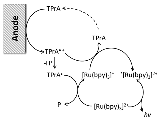
Figure 18. Mechanism of ECL in the [Ru(bpy) 3 ] 2+ tripropylamine (TPrA) system. [79]
