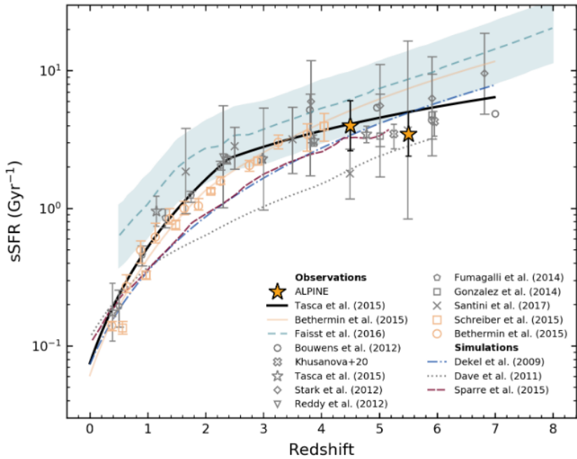
Fig. 11. SSFR evolution with redshift. Results of various observations and numerical simulations are shown (Dekel et al. 2009; Davé et al. 2011; Sparre et al. 2015). Gray symbols are based on FUV data (Bouwens et al. 2012; Khusanova et al. 2020; Tasca et al. 2015; Stark et al. 2013; Reddy et al. 2012; Fumagalli et al. 2014; González et al. 2014; Santini et al. 2017). Orange symbols are based on the rest-frame FIR data (Schreiber et al. 2015; Béthermin et al. 2015). The orange filled stars show this paper's results. The solid line shows the fit to results by Tasca et al. (2015), the shaded area and the dashed line show the results coming from the observations of EW(H \alpha ) in COSMOS (Faisst et al. 2016).
