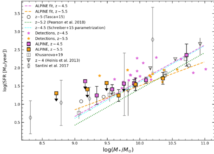
Fig. 10. Main sequence of star-forming galaxies at z \sim 4.5 and z \sim 5.5 . The filled squares are the measurements of average SFR from stacks; the open symbols are results from the literature; the magenta and orange lines are the fits of the main sequence at z \sim 4.5 and z \sim 5.5 respectively; the cyan and green lines are the fits of the main sequence from the literature. The colored stars are the individual galaxies in ALPINE with FIR continuum detections at >3\sigma .
