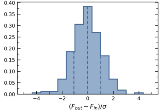
Fig. 1. Comparison of injected and recovered fluxes from stacking. The vertical dashed lines correspond to 16th, 50th and 84th percentiles of the distribution ( -1.08 , -0.02 , 1.03 ).
