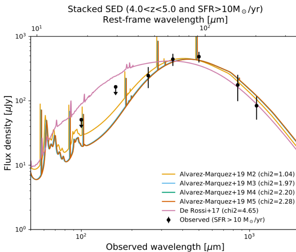
Fig. A.1. Comparison of the chosen dust SED templates with the stacks of Herschel data at 4 < z < 5 . The black symbols are stacked Herschel data and the solid lines are templates from the literature.
