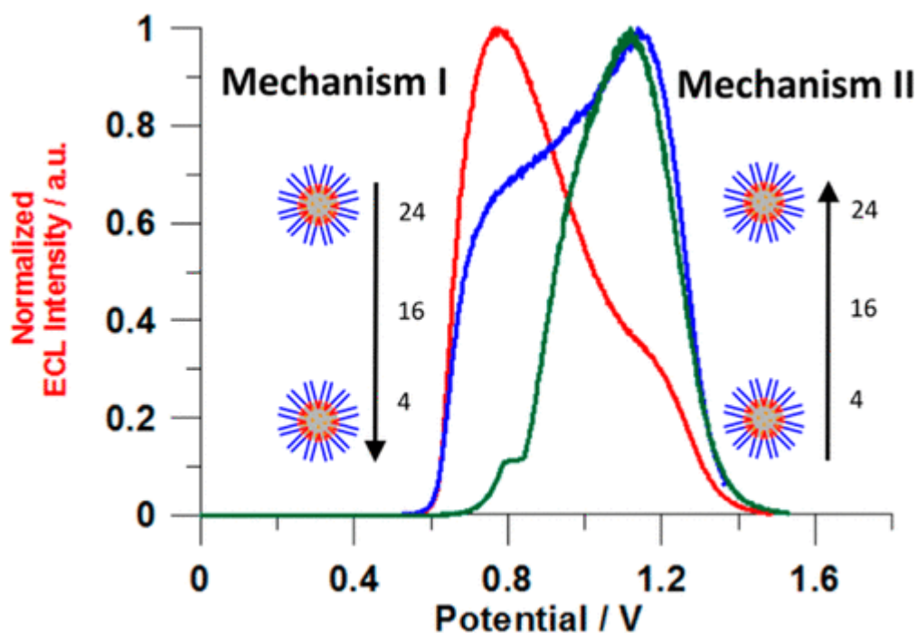
Figure 8. Normalized ECL intensity vs potential curves of Ru@NP3 (red), Ru@NP4 (blue), and Ru@NP6 (green) (Ru/NP = 4, 16, 24) in 100 mM PB solutions, with 30 mM DBAE as coreactant: scan rate 0.1 \text{ V s}^{-1} ( E vs SCE), PMT bias 750 V.
