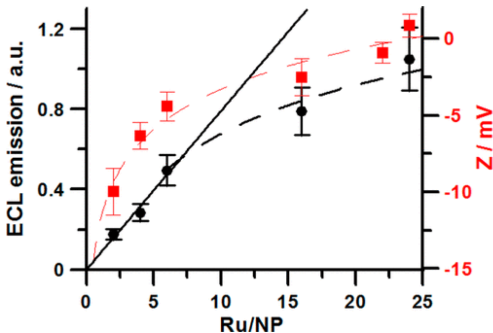
Figure 9. Integrated ECL intensity (black dots) measured during chronoamperometric experiments with Ru@NP1-6 (Ru/NP = 2–24). Conditions: 100 mM PB solutions, 30 mM DBAE as coreactant, applied potential =1.4 V for 0.5 s ( E vs SCE), PMT bias 750 V, and \zeta -potential (red dots) as a function of the doping.
