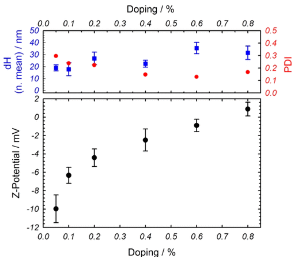
Figure 3. \zeta -Potential (lower panel), hydrodynamic diameter (by number mean), and PDI (polydispersion Index) (upper panel) of samples Ru@NP1–6 vs Rubpy–TES doping percentage. Conditions: [Ru@NP] = 4 \mu M, [KCl] = 1 mM, [phosphate buffer] = 1 mM, pH 7.0, T = 25 °C (all samples were filtered with a 200 nm RC syringe filter). Hydrodynamic diameter and \zeta -potential values are reported in Table 1; error bars were calculated as standard deviations of 10 measurements.
