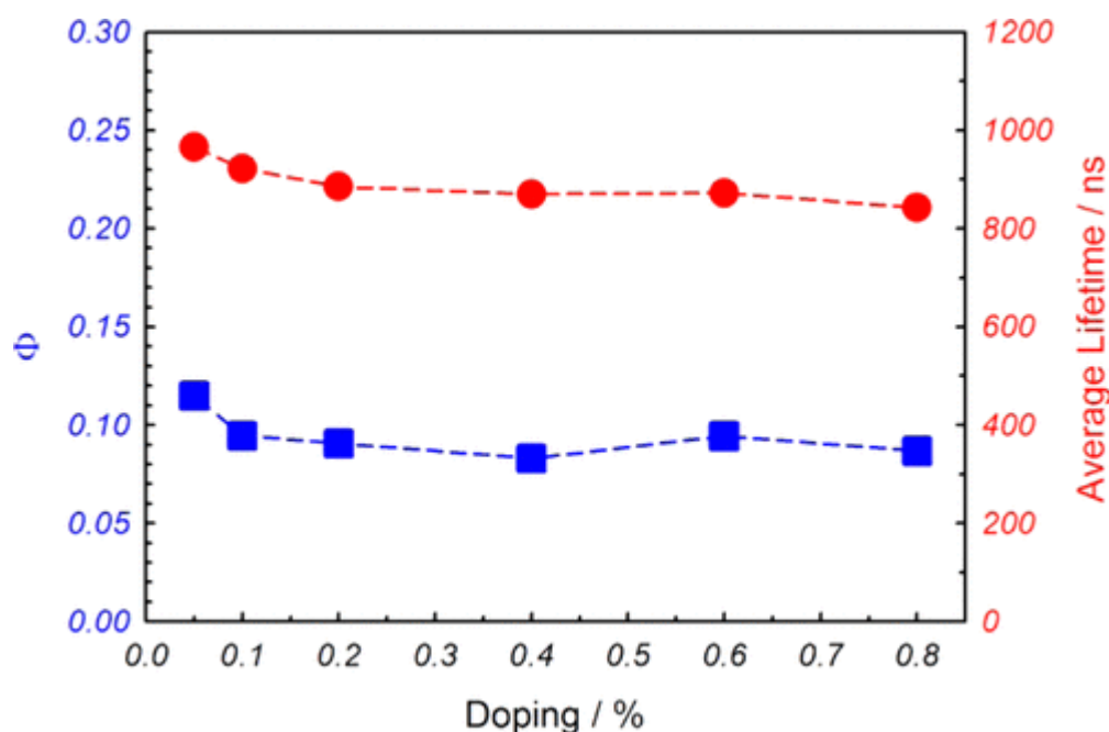
Figure 5. Luminescence quantum yields (blue) and average excited state lifetimes (red) values for samples Ru@NP1–6 in aerated conditions (water, \lambda_{\text{ex}} = 460 \text{ nm} ). For reference compound \text{Ru}(\text{bpy})_3^{2+} : \Phi = 0.03 ; \tau = 370 \text{ ns} .
