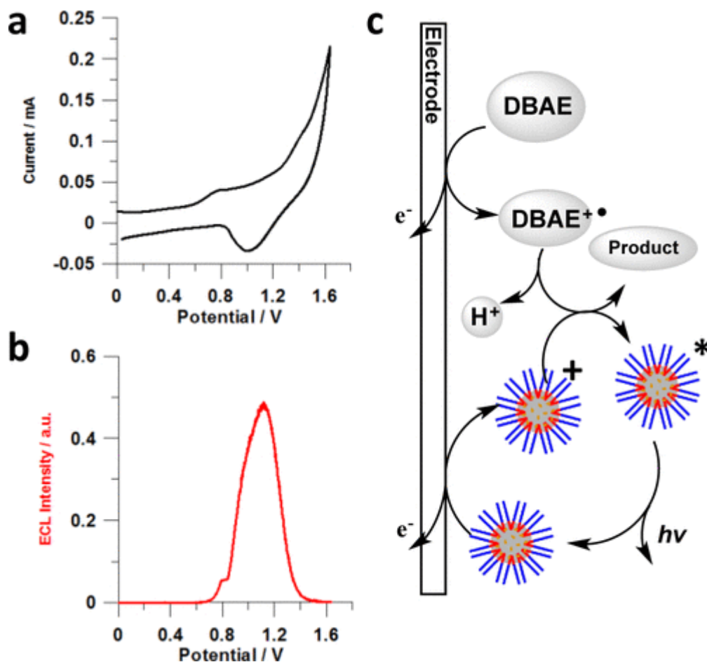
Figure 7. Cyclic voltammetry (black trace panel a) and ECL intensity (red trace panel b) vs potential curves of \text{Ru@NP6} ( \text{Ru}/\text{NP} = 24 ), in PB 100 mM solutions, with 30 mM DBAE as coreactant: scan
