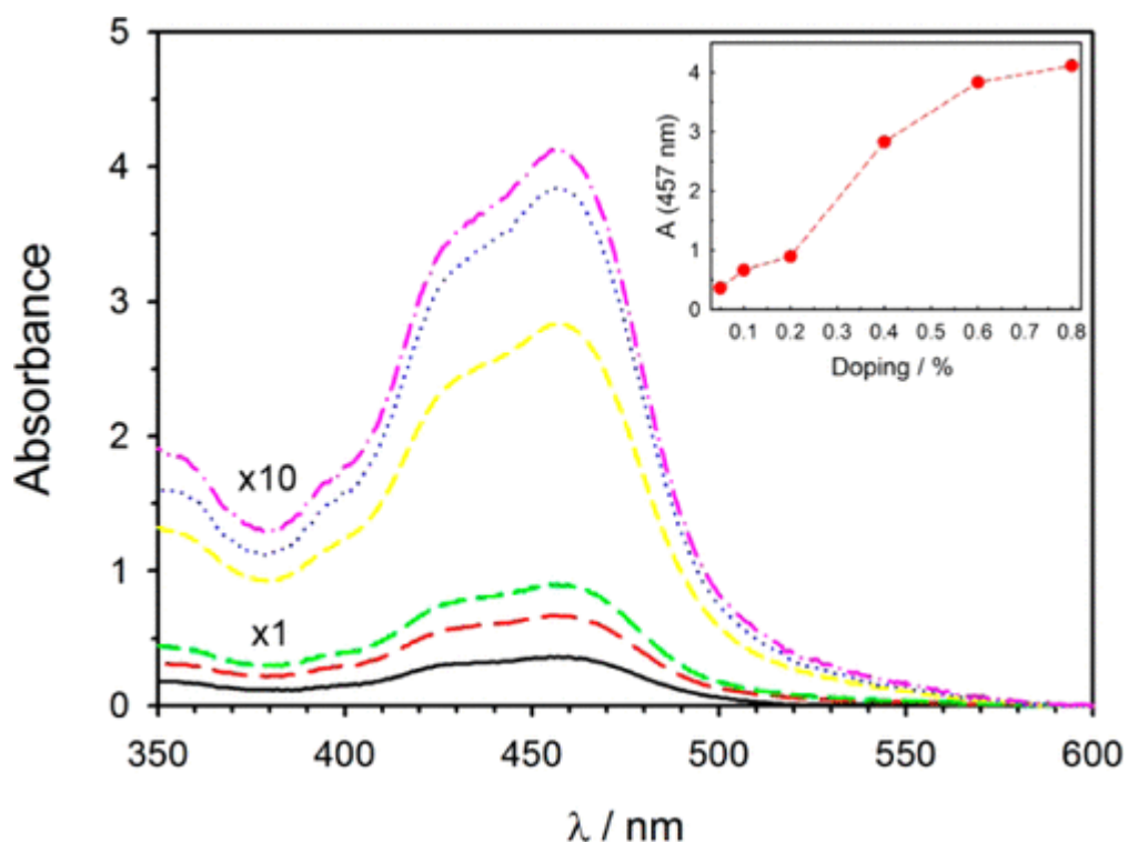
Figure 4. Absorption spectra of samples Ru@NP (1, black; 2, red; 3, green; 4, yellow; 5, blue; 6, pink). Conditions: water, [\text{Ru@NP}] = 10 \mu\text{M} filtered with a RC 200 \mu\text{m} filter. Samples Ru@NP1–3 , cuvettes with optical path 1 cm; samples Ru@NP4–6 , cuvettes with optical path 0.1 cm. Inset: absorbance at 457 nm vs % doping.
