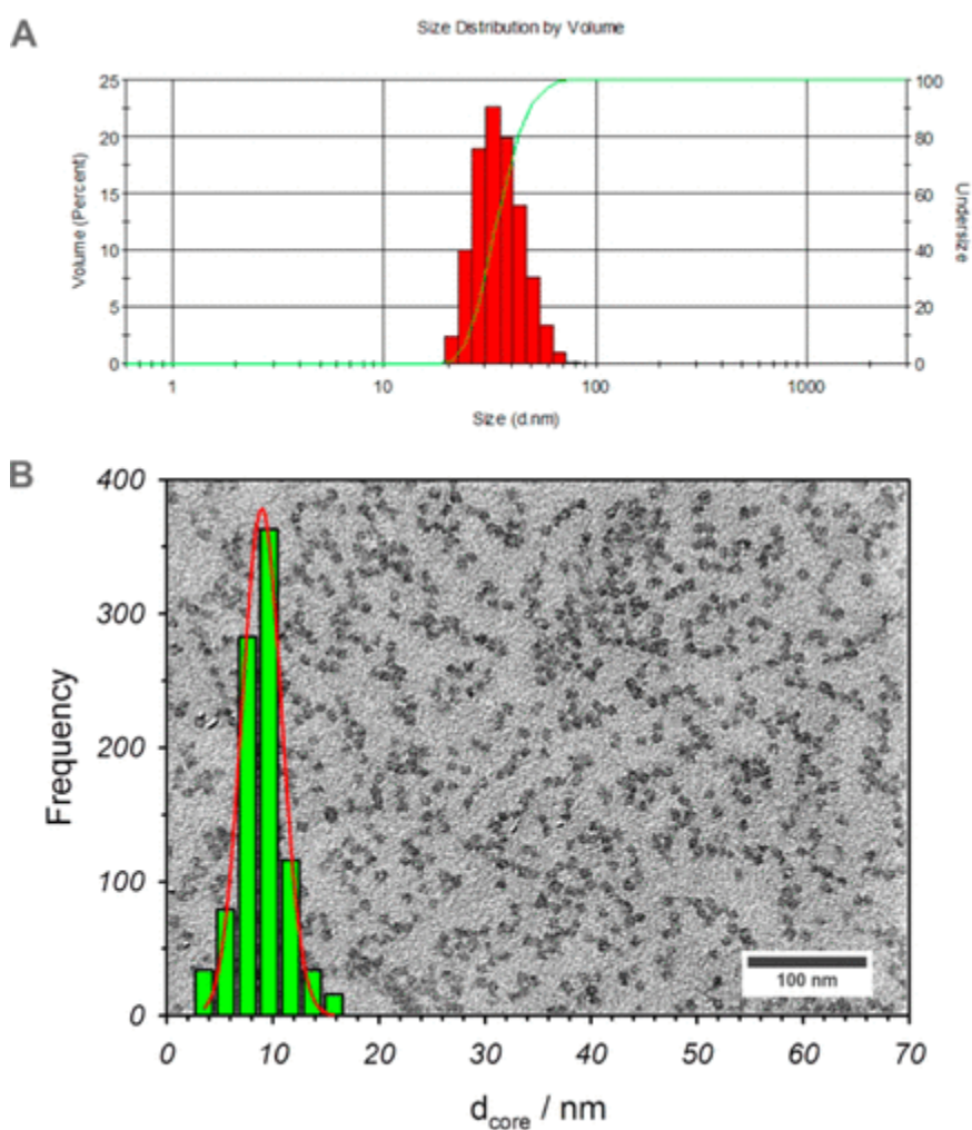
Figure 2. (A) Hydrodynamic diameter distribution of DDSNs ( Ru@NP4 ) in water. (B) TEM image and silica core diameter distribution ( Ru@NP4 ).
