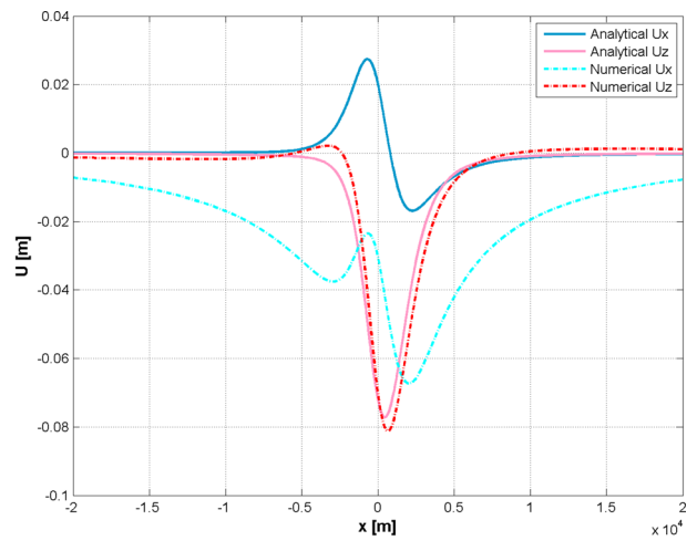
(b) Method 1, Distance 1.5 radii, \Delta P = -20 MPa
