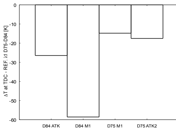
Figure 44. Temperature difference compared to the respective REFERENCE case \lambda 1.0 STD cam – Bores 75 mm and 84 mm – CR 9.5
