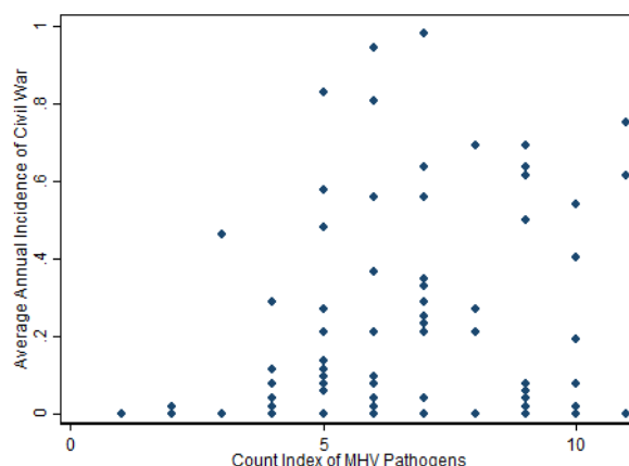
Figure A.1: Disease Environment and Conflicts
