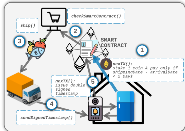
Figure 2: Programmability in M2M payments. A Direct Integration type of payment where a coin is staked and released only if a condition is met, i.e. goods are delivered in time
