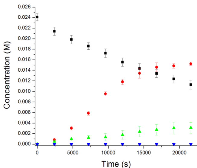
Figure 1. Decomposition of azocumene (black) and formation of the cumyl-TEMPO adduct in the presence of TEMPO+BF 4 - (25 mM) and Me 4 N + AcO - (25 mM) in acetonitrile at 50 °C under an atmosphere of argon (red), air (green) or O 2 (blue).
