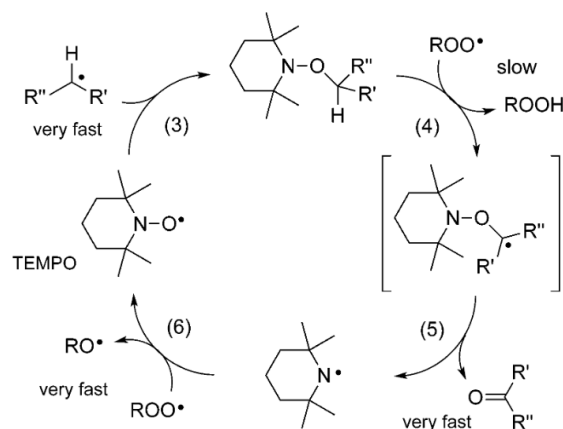
Scheme 1. Proposed Mechanism of Hindered Amine Light Stabilizer Activity
