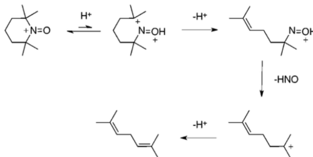
Scheme 3. Proposed Mechanism for the Decomposition of TEMPO + in the Presence of Strong Acid
