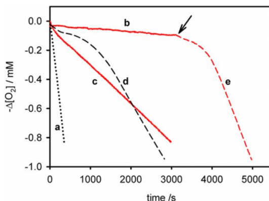
Figure 5. O_2 consumption during the autoxidation of styrene (4.3 M) in acetonitrile containing 1% H_2O initiated by AIBN (0.05 M) at 30 °C (a) and corresponding experiments carried out in the presence of TEMPO (13 \mu M ) and acetic acid (43 mM) (b), acetic acid (43 mM) and Oct_4NBF_4 (0.13 M) (c), acetic acid (43 mM) and HBF_4 (43 mM) (d), and acetic acid (43 mM) with HBF_4 (43 mM) added at the time indicated by the arrow (e).
