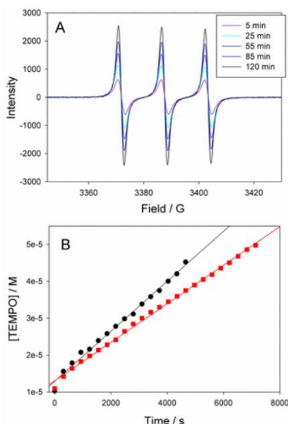
Figure 4. TEMPO formation during the autoxidation of styrene (4.3 M) in acetonitrile initiated by AIBN (50 mM) at 30 °C in the presence of TEMPO + BF 4 - (0.66 mM). Top: Representative EPR spectra. Bottom: Rate with (black) and without (red) added acetic acid (35 mM).
