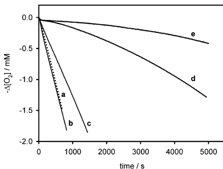
Figure 2. O 2 consumption during the autoxidation of styrene (4.3 M) in acetonitrile initiated by AIBN (0.05 M) at 30 °C (a, dotted line) and corresponding experiments carried out in the presence of 13 μM of either TEMPO + BF 4 - (b,d) or TEMPO (c,e) with (d,e) or without (b,c) acetic acid (43 mM).
