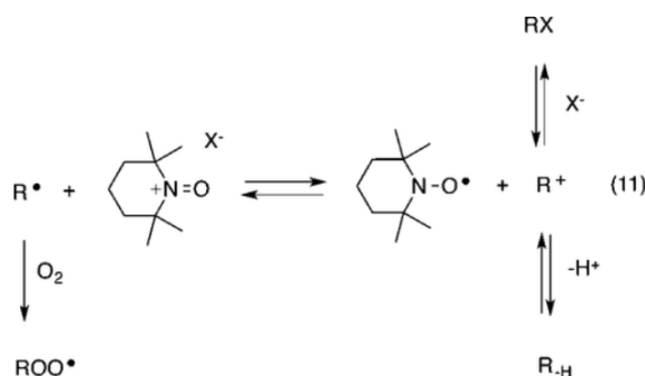
Scheme 4. Reactions Influencing the Reversibility of the Electron Transfer between TEMPO + and an Alkyl Radical
