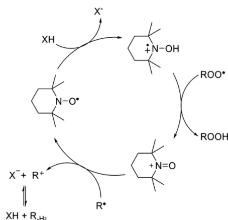
Scheme 5. Proposed Mechanism of Acid-Catalyzed RTA Activity of Nitroxides
