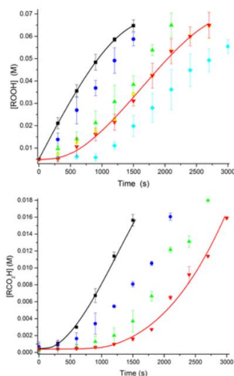
Figure 6. Hydroperoxide (top) and acid (bottom) formation in the autoxidation of light paraffin oil at 160 °C initiated by 5 mM tetralin hydroperoxide (black) and inhibited by 40 \mu\text{M} 2 (red) with 4 mM palmitic acid (yellow), 40 mM palmitic acid (light blue), 4 mM 2,4,6-( t -Bu) 3 pyridine (green), or 40 mM 2,4,6-( t -Bu) 3 pyridine (dark blue).
