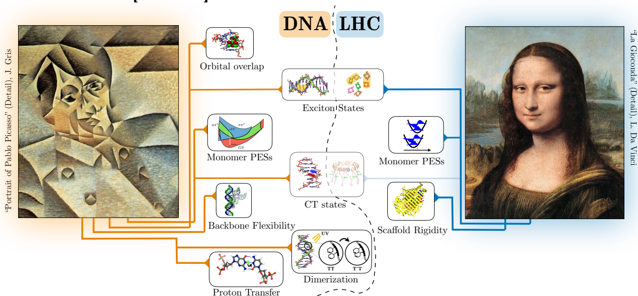
Figure 5: Different “faces” of the modeling when applied to LH-like and DNA-like multichromophoric systems. On the right, a perfect face (“La gioconda” by L. da Vinci), which represents the modeling of LH complexes, with approximations which can be controlled and tuned. On the left, a peculiar face, (“Portrait of Pablo Picasso”, by J. Gris): one identifies various components (eyes, nose, mouth, etc.) but the face as a whole is not easy to read. This represents the present challenges in the modeling of DNA-like multichromophoric systems.
