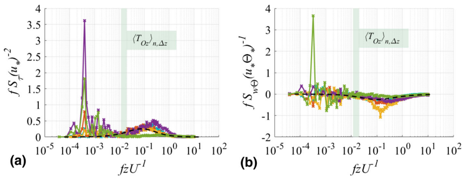
Fig. 6 Non-dimensional spectra of \tau (a) and w\Theta (b) as a function of the non-dimensional frequency for all tower levels (0.5 m in blue, 2 m in red, 5 m in yellow, 10 in purple, and 20 m in green). Black dashed lines represent the reference spectra from Eq. 30. The green vertical bands describe the variability within the 20-m layer of the mean value of the Ozmidov scale through the night
