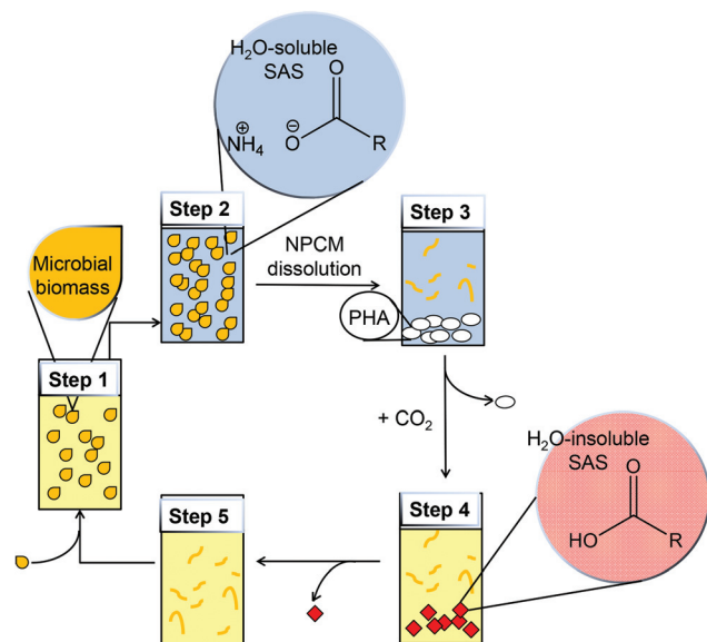
Fig. 6 Use of \text{CO}_2 as a pH-trigger for recovering ammonium carboxylate SAS after the dissolution of NPCM.
