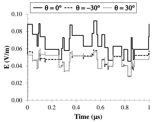
Fig. 13. Far-field envelopes at 1 m-distance, in correspondence of the three radiation maxima of Fig. 12(a).
