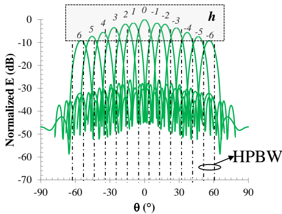
Fig. 7. Ideal full exploitation of a 16-dipole TMA sideband radiation, when considering up to the sixth harmonic, for multiple tags powering.
