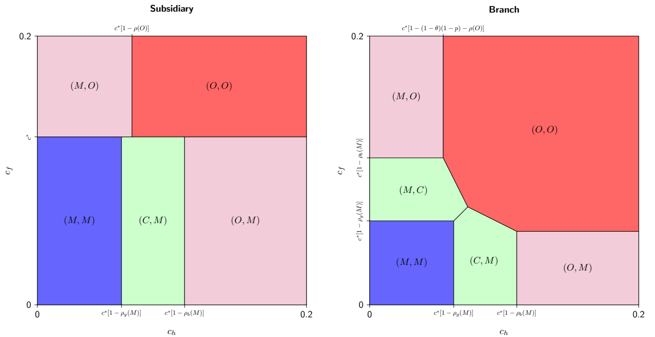
Figure 2: Equilibrium supervisory decisions under national supervision of a subsidiary and a branch, as functions of the monitoring costs c_h and c_f . The parameters are \theta = 1/2 , p = 3/4 , R = 1.5 .
