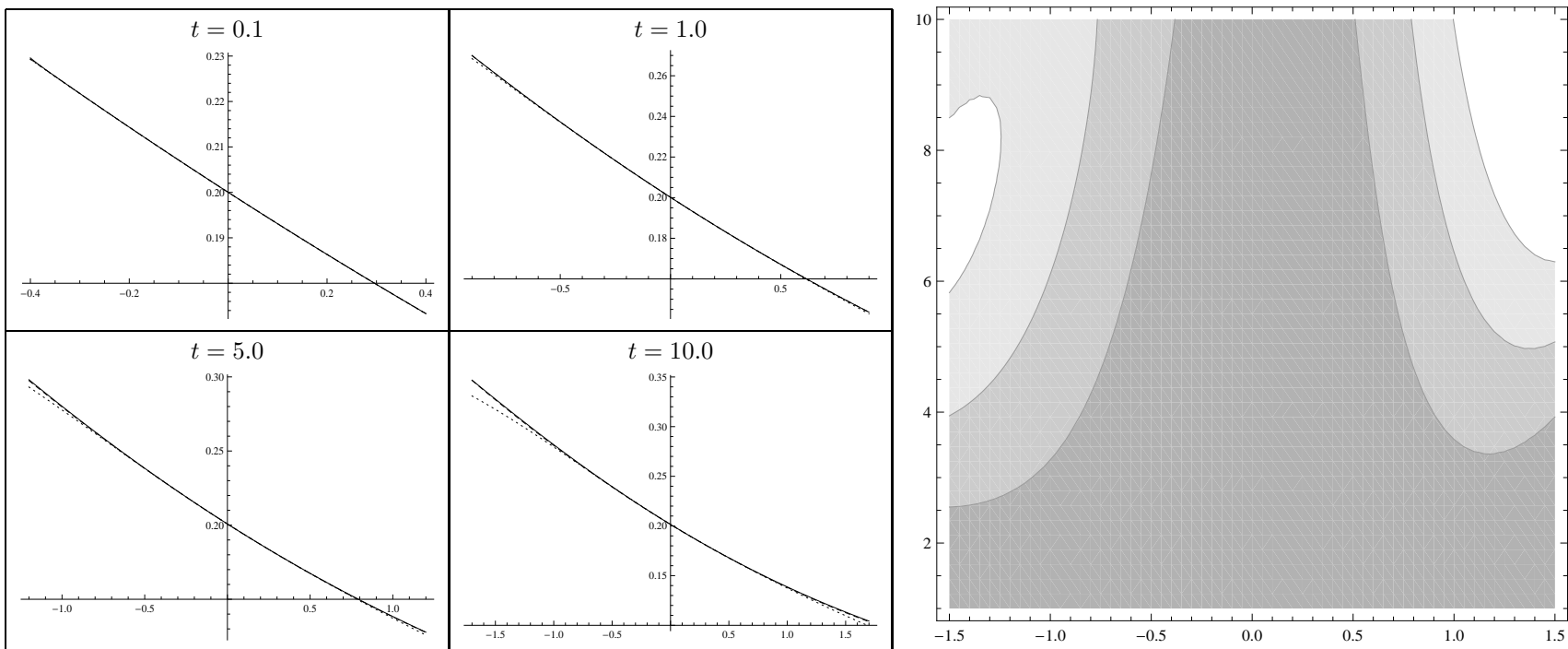
Figure 1: LEFT: Implied volatility in the CEV model (5.1) is plotted as a function of log-moneyness ( k-x ) for four different maturities t . The solid line corresponds to the implied volatility \sigma obtained by computing the exact price u using (5.3) and then by solving (3.3) numerically. The dashed line (which is nearly indistinguishable from the solid line) corresponds to our third order implied volatility approximation \bar{\sigma}_3 , which we compute by summing the terms in (5.2). The dotted line corresponds to the implied volatility expansion \sigma^{HW} of Hagan and Woodward (1999), which is computed using (5.4). RIGHT: We plot the absolute value of the relative error |\bar{\sigma}_3 - \sigma|/\sigma of our third order implied volatility approximation as a function of log-moneyness ( k-x ) and maturity t . The horizontal axis represents log-moneyness ( k-x ) and the vertical axis represents maturity t . Ranging from darkest to lightest, the regions above represent relative errors of < 0.3\% , 0.3\% to 0.6\% , 0.6\% to 0.9\% and > 0.9\% . We use the following parameters: \beta = 0.3 , \delta = 0.2 , x = 0.0 .
