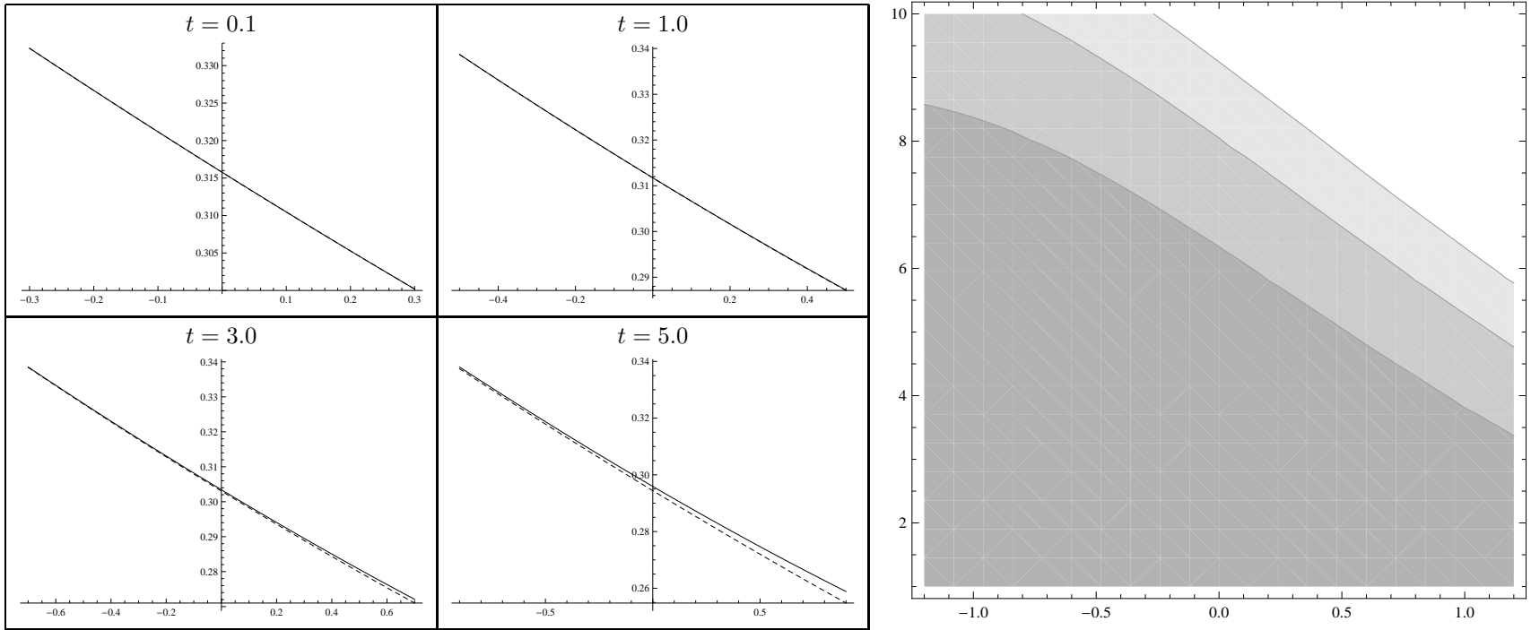
Figure 3: LEFT: Implied volatility in the 3/2 stochastic volatility model (5.9) is plotted as a function of log-moneyness (k-x) for four different maturities t . The solid line corresponds to the implied volatility \sigma , obtained by computing the exact price u using (5.12) and then by solving (3.3) numerically. The dashed line corresponds to our third order implied volatility approximation \bar{\sigma}_3 , which we compute by summing the terms in (5.10). RIGHT: We plot the absolute value of the relative error |\bar{\sigma}_3 - \sigma|/\sigma of our third order implied volatility approximation as a function of log-moneyness (k-x) and maturity t . The horizontal axis represents log-moneyness (k-x) and the vertical axis represents maturity t . Ranging from darkest to lightest, the regions above represent relative errors of < 1\% , 1\% to 2\% , 2\% to 3\% and > 3\% . We use the following parameters: \kappa = 0.25 , \theta = 0.1 , \delta = 0.8 , \rho = -0.85 x = 0.0 , y = \log \theta .
