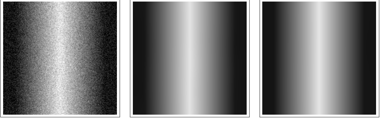
Figure 7: Example 5: restoration results obtained by the S_1H-\ell_2 model (center), SNR = 37.14 , and the associated CNC-NS- \ell_2 model (right), SNR = 45.97 , applied to the piecewise affine test image roof corrupted by space-invariant Gaussian blur with parameters (\mathbf{band}, \mathbf{sigma}) = (9, 2) and by AWGN with standard deviation \sigma = 20 (left).
