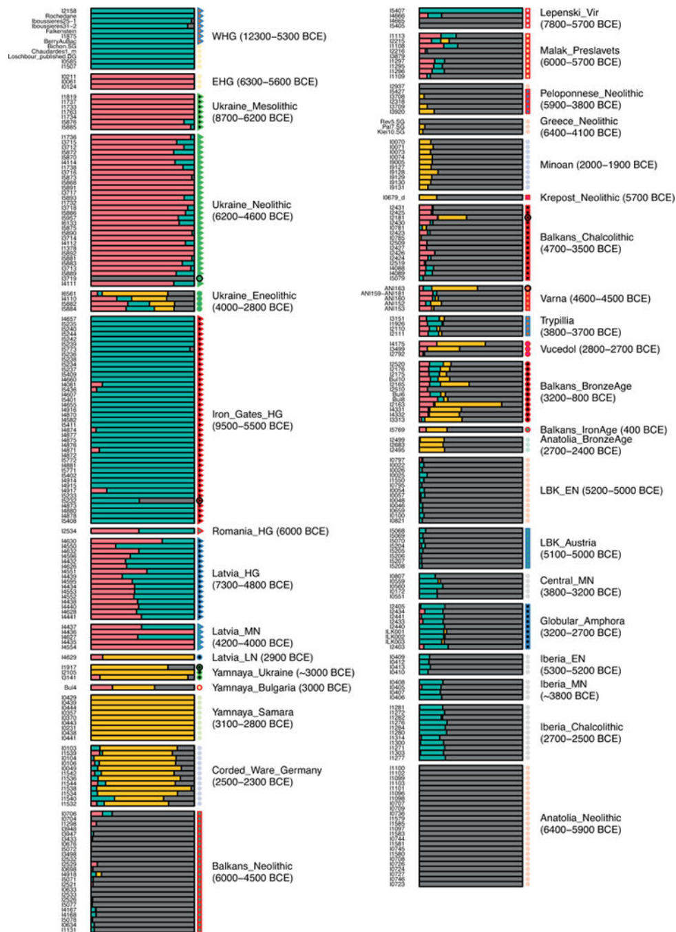
Extended Data Figure 2. Supervised ADMIXTURE analysis modeling each ancient individual (one per row), as a mixture of populations represented by clusters that are constrained to contain Anatolian Neolithic (grey), Yamnaya from Samara (yellow), EHG (pink) and WHG (green)
