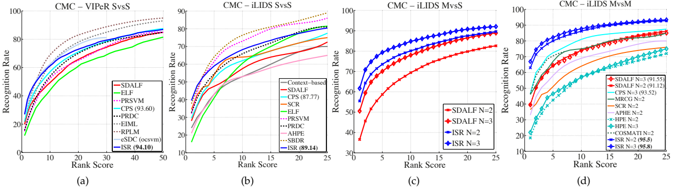
Fig. 4: Comparative performance evaluation on VIPeR and i-LIDS. (a) SvsS on VIPeR. (b) SvsS on i-LIDS. (c) MvsS on i-LIDS ( N \in \{2, 3\} ). (d) MvsM on i-LIDS ( N \in \{2, 3\} ). Dashed curves distinguish techniques that set aside a portion of the dataset for learning. In the legends we report the normalized area under the CMC curve (nAUC), when available.
