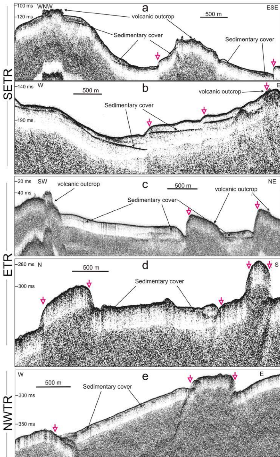
Fig. 9 CHIRP profiles across the main volcanic and tectonic features observed offshore Terceira (location in Fig. 1). The magenta arrows indicate fault scarps. On CHIRP profiles, the base of the recognizable sedimentary cover is indicated by black arrows , varying between some meters (profiles a, c, d and e) up to 15 m (profile b)
