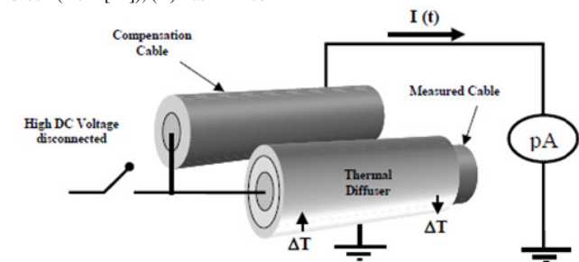
Figure 7. TSM space charge measurements on cables in double capacitor configuration: the measurement is performed on the measured cable after disconnecting the dc source. (after [38]).
