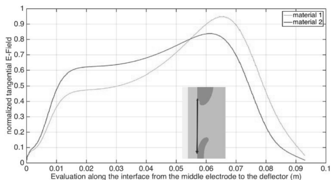
Figure 4. Normalized tangential electric field at steady state in a HVDC joint with two different insulation materials: material 2 has temperature dependence of conductivity more similar to XLPE than material 1. After [22].
