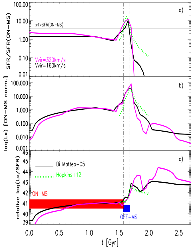
FIG. 3.— Comparison of our results with predictions of hydrodynamical models that simultaneously follow star formation and the growth of black holes during a galaxy-galaxy merger (Di Matteo et al. 2005, Hopkins et al. 2012). a) To define the simulated merger/starburst phase we report the SFR history of the models normalized to the pre-merger phase. The temporal window where (\text{SFR})/(\text{SFR pre-merger}) is larger than a factor 4 for all models is marked by the two vertical dot-dashed lines. b) Evolution of the X-ray luminosity with time. c) Evolution of the X-ray luminosity to SFR ratio, as a function of time. Two different values of the virial velocity of the collisional galaxies are considered in the Di Matteo et al. (2005) model ( v=160\text{km/s} black lines, v=320\text{km/s} magenta lines). Our results are presented as a red rectangle for the pre-merger phase (corresponding to our MS normal star-forming sources) and as a blue region for the merger phase (i.e. our starburst sample). The width of L_X/\text{SFR} from our data spans the full range covered in all mass bins (see Fig. 1, bottom panel).
