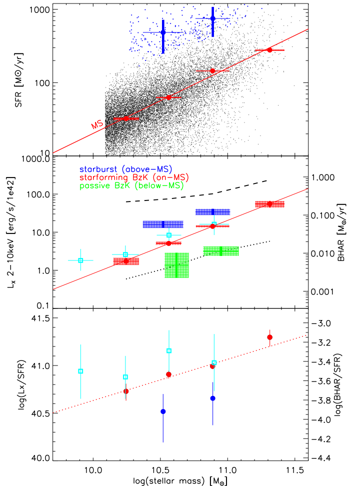
FIG. 1.— Top panel: The mass-SFR relation. We report the sBzK sample with their SFR(UV) (black points), while the corresponding average SFR(IR+UV) derived from the PACS stacking analysis are reported as red filled circles (Rodighiero et al. 2014). The linear fit provides an MS relation as \log[SFR] = 0.89(\pm 0.09) \times \log[M_*] + 14.02 . We also show the starburst sample (blue points) with the corresponding average SFR(IR+UV) in the two mass bins (errors on average SFR are the standard deviation of the SFR distribution within each mass bin). Middle panel: stellar mass-average L_X relation at 1.5 < z < 2.5 from our X-ray stacking analysis. Shaded colour regions are the results for the three samples: starburst (blue), main sequence (red) and quiescent sources (green). We provide a fit for the MS sample (solid red line, \log[L_X] = 1.40(\pm 0.09) \times \log[M_*] - 14.11 ). The open cyan squares are the results of M12 in GOODS-S, scaled to the same K-correction adopted in this work. The dashed and dotted black lines represent the average L_X of detected and stacked X-ray sources in the MS, respectively. Bottom panel: L_X/SFR relation for MS (red) and starburst (blue). The dotted line is a linear fit to the relation for the MS sample ( \log[L_X/SFR] = 0.43(\pm 0.09) \times \log[M_*] + 35.6 ) and the open cyan squares are again the results of M12. In each panel the width of the stacked data along the x-axis represents the RMS of the mass distribution in each bin.
