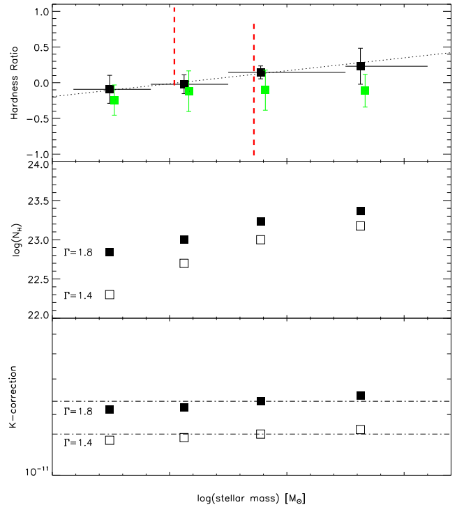
FIG. 2.— Top panel : Stellar mass – HR relation at 1.5 < z < 2.5 for the MS-sBzK stacked sample (filled black squares). The dotted line is a linear fit to the distribution ( \text{HR} = 0.31 \times \log[M_*] - 3.3 ). The vertical red dashed lines show the marginal constraints that we can derive for the starbursts, basically consistent with the MS. The values for the detected sources are also reported (green squares). Middle panel : Derived N_H values for two different assumptions of the X-ray spectral slope \Gamma . Bottom panel : Final K-corrections for the two different values of \Gamma turn to be almost constant with mass. We adopt a constant value of \Gamma=1.4 and N_H=22 .
