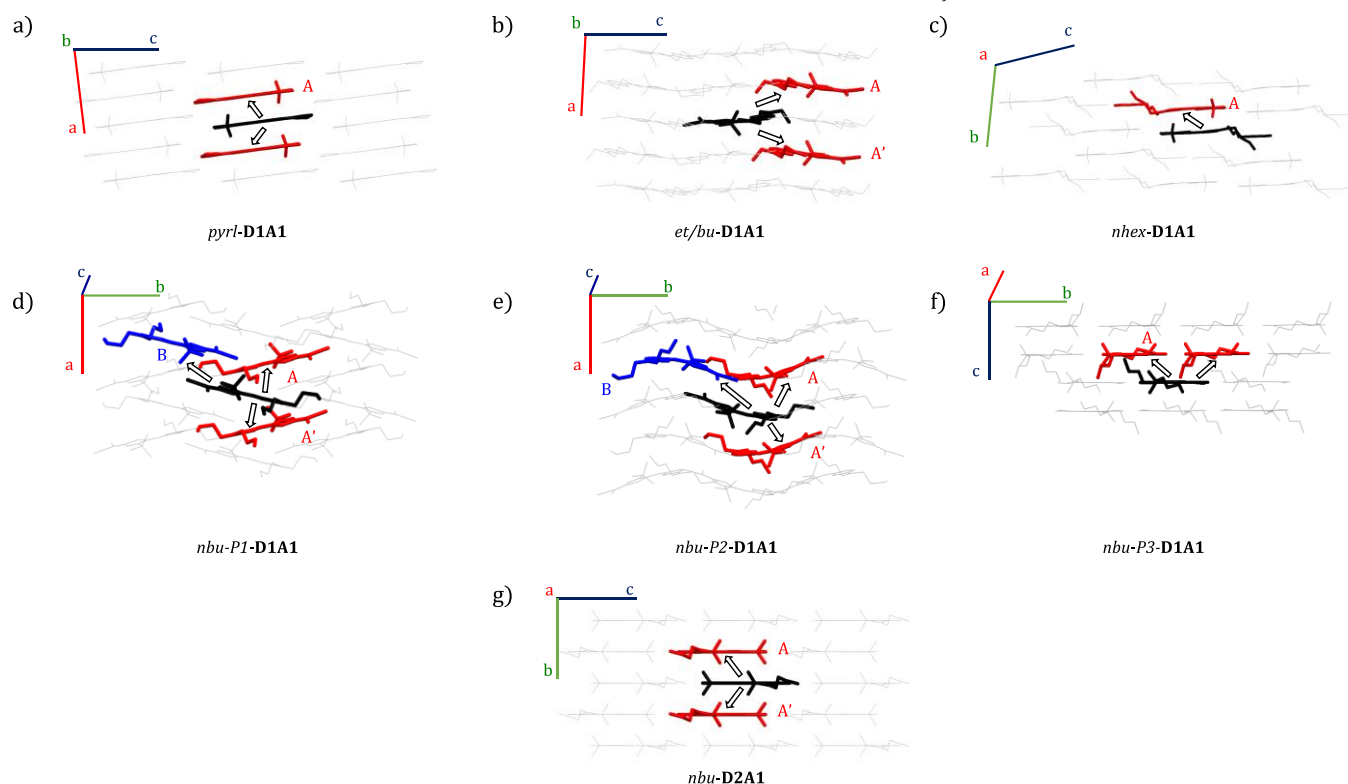
Figure 6: Supercells of the crystal structures for D1A1 (a-f) and D2A1 (g) classes. For each crystal (a – pyrl -, b – et/bu -, c – nhex -, d – nbu-P1 -, e – nbu-P2 -, f – nbu-P3-D1A1 , g – nbu-D2A1 ) is reported a schematic view of the charge pathways from the central molecule (black) to those nearest neighbor molecules (red) showing large V_{ij} ( V_{ij} > 10 meV). For nbu-P2 - and nbu-P1-D1A1 crystals (d, e), the molecule highlighted in blue represents, together with the black one, dimer B (see text), namely the inter-column coupling (see text). Letters (A, A' and B) label non-equivalent nearest neighbor dimers.
