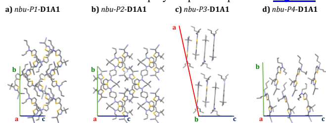
Figure 5: Crystal structures (supercell) of nbu-Pn-D1A1 polymorphs as obtained in the current work, namely a) nbu-P1 - (chloroform, XRD at room temperature), b) nbu-P2 - (chloroform, XRD at 100 K), c) nbu-P3-D1A1 (mesitylene, XRD at 100K); d) nbu-P4-D1A1 as reported in Ref. 28
