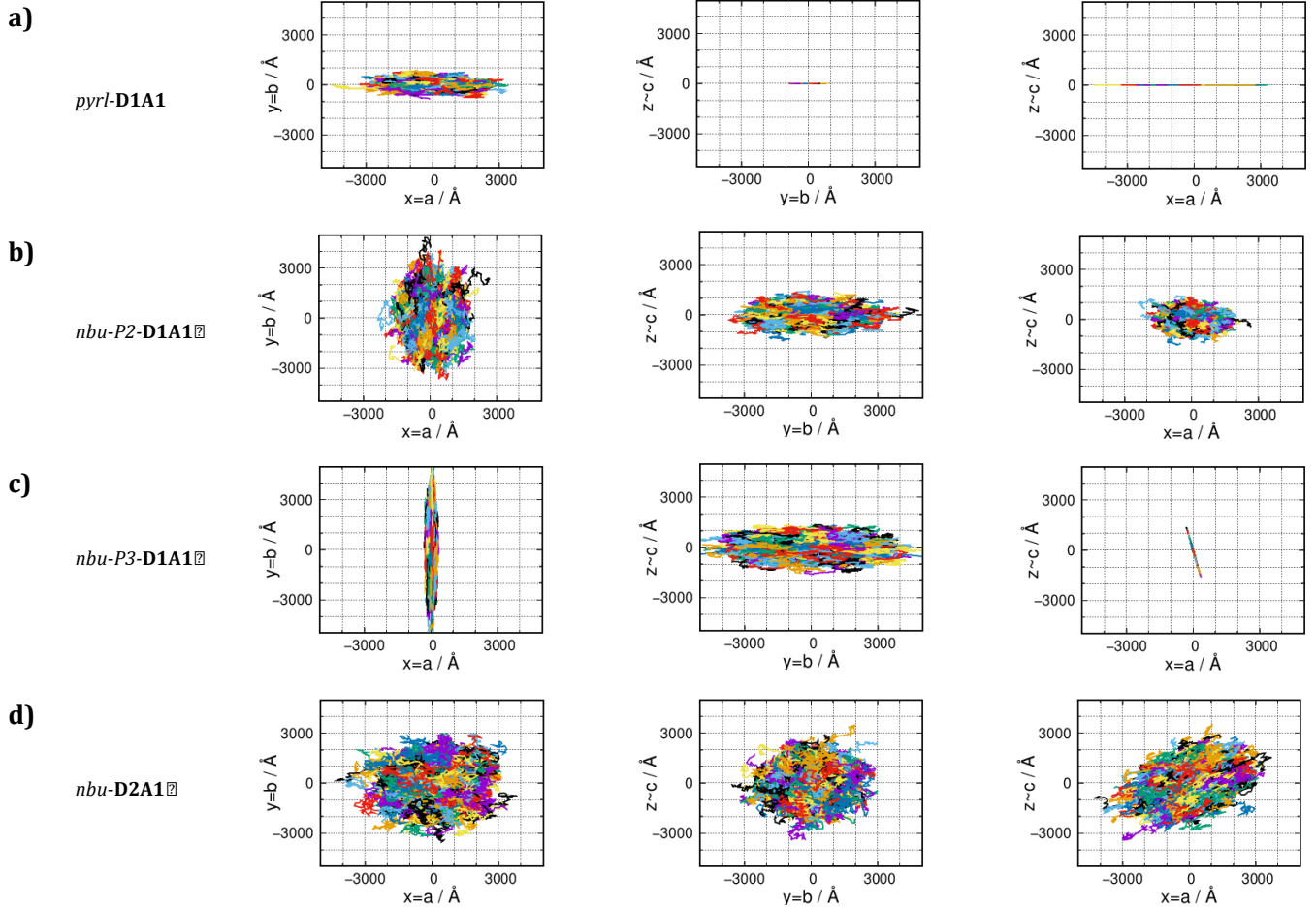
Figure 7: Plot of 1000 kMC trajectories (each consisting of 10^5 steps) for each D1A1 and D2A1 class (from top to bottom: pyrl- , nbu-P2- , nbu-P3-D1A1 and nbu-D2A1 ). Trajectories are reported for the three Cartesian planes, namely yx , zy and zx (crystallographic axes are reported as well).
