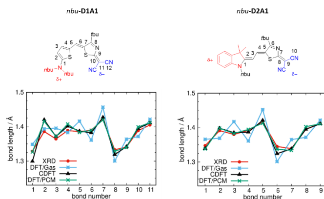
Figure 2: Bond structures and BLA paths (as defined by bond numbering) for nbu-D1A1 (left) and nbu-D2A1 (right) merocyanine – upper panels ( nbu-D1A1 , known also as HB238 ). 3 Bond lengths (Å) from XRD data (red lines), DFT ( \omega B97X-D3/6-311G**, gas phase, blue lines), C-DFT (CAM-B3LYP-D3/6-311G**, gas phase,
