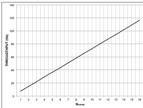
Fig. 14. In the worst case, where publishers update a large set of triples (i.e., 100 triples), the SUB Engine running on a 16 cores system is still able to notify (i.e., with a notification consisting of 200 bindings) more than 100 subscribers in one second
