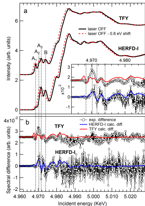
Figure 4. Effect of LSPR excitation in full XANES acquired in TFY and HERFD-I on N- \text{TiO}_2 /Au. Panel a: experimental (black continuous line) and red-shifted (red dashed line) laser off spectra. Panel b: TFY and HERFD-I laser on - laser off differences of experimental data (black dotted line) and generated shifted - unshifted differences of TFY (red line) and HERFD-I (blue line)
