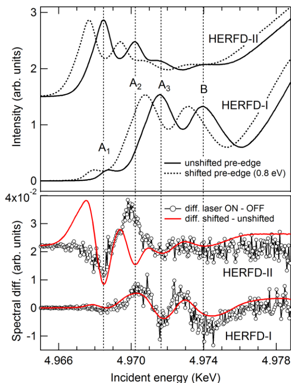
Figure 5. The upper panel shows experimental (continuous line) and red-shifted (dashed line) laser off HERFD-II and HERFD-I pre-edges of N- \text{TiO}_2 /Au. The bottom panel displays experimental laser on - laser off differences (black line) compared to generated shifted - unshifted differences (red line) for HERFD-II and HERFD-I. HERFD-I laser variations are reproduced fairly well by red-shifting experimental data. On the contrary, HERFD-II laser variations are not compatible with a red-shift of transitions.
