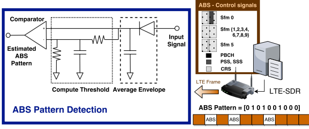
Fig. 6. ABS detection enabled by an envelope detector, which smoothens out the fluctuations, and a comparator, which detects whether the power level exceeds a pre-defined threshold [35]. The LTE interference is generated using a USRP B210 empowered with srsLTE (for further details, see Section 3.2).
