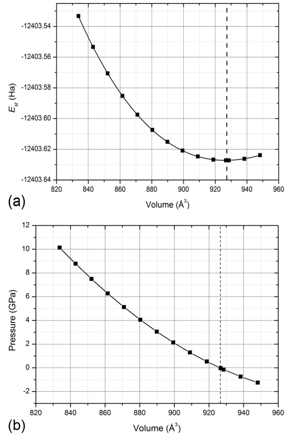
FIGURE 3. (a) E_{st}(V) in Hartree units and (b) P(V) plots of muscovite obtained from ab initio calculations. The dashed lines helps in distinguishing compression regime (on the left) and expansion (on the right).
